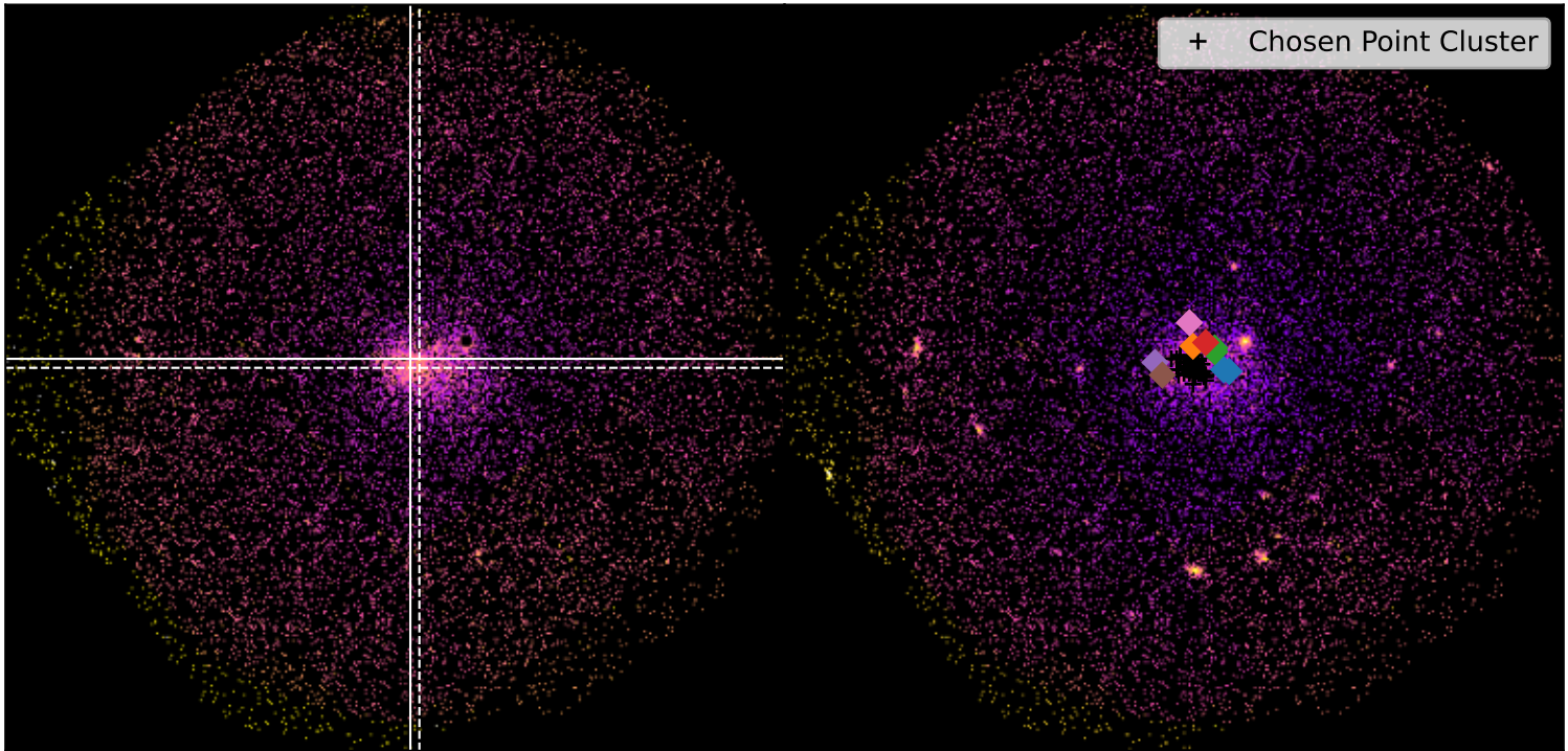
SDSSXCS-893 - Combined 0.5-2.0keV ratemapSDSSXCS-893 - Combined 0.5-2.0keV ratemap
