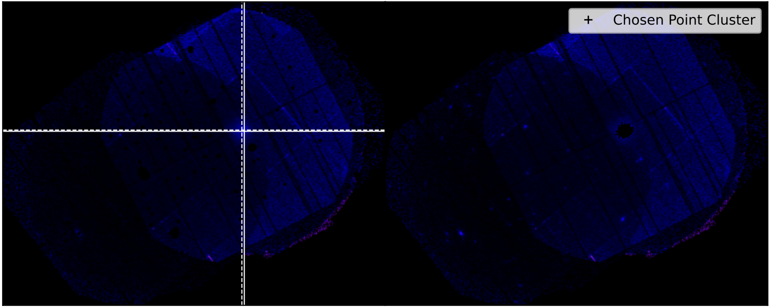
SDSSXCS-907 - Combined 0.5-2.0keV ratemapSDSSXCS-907 - Combined 0.5-2.0keV ratemap
