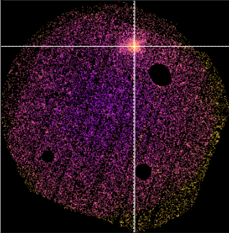
SDSSXCS-913 - Combined 0.5-2.0keV ratemapSDSSXCS-913 - Combined 0.5-2.0keV ratemap
