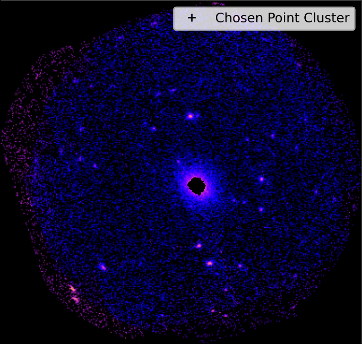
SDSSXCS-9803 - Combined 0.5-2.0keV ratemap
