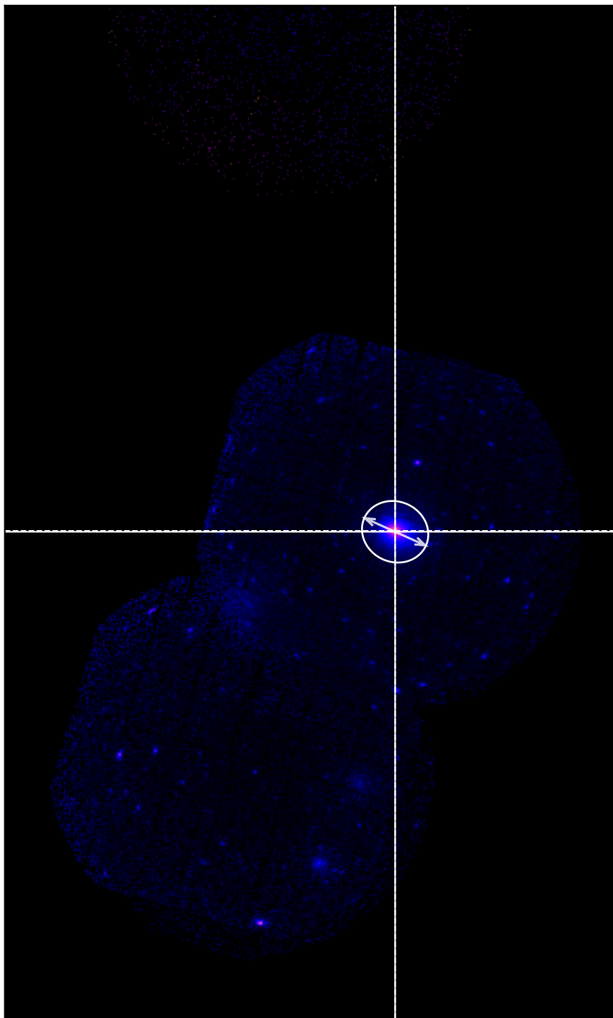
SDSSXCS-1137 - Combined 0.5-2.0keV ratemap
