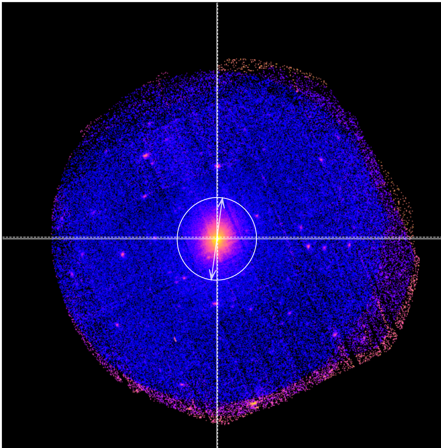
SDSSXCS-78 - Combined 0.5-2.0keV ratemap
