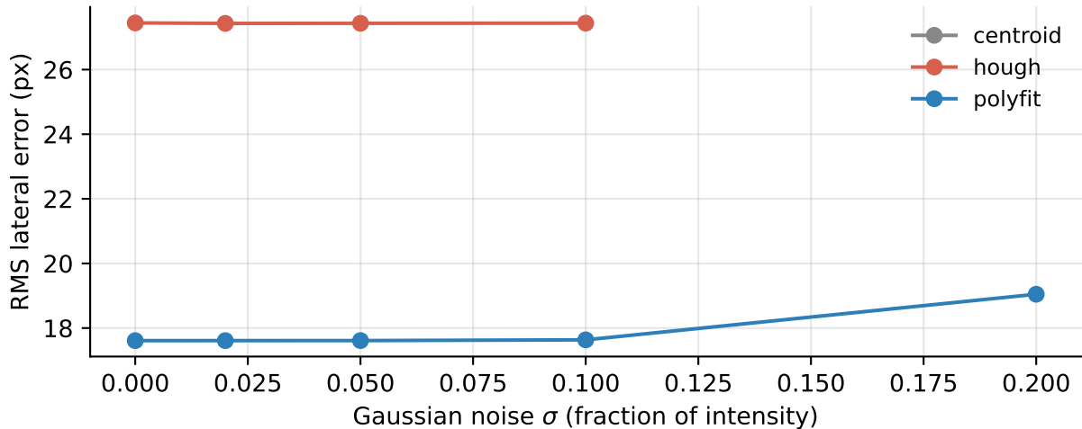
Noise robustness on the oval (PID controller)
