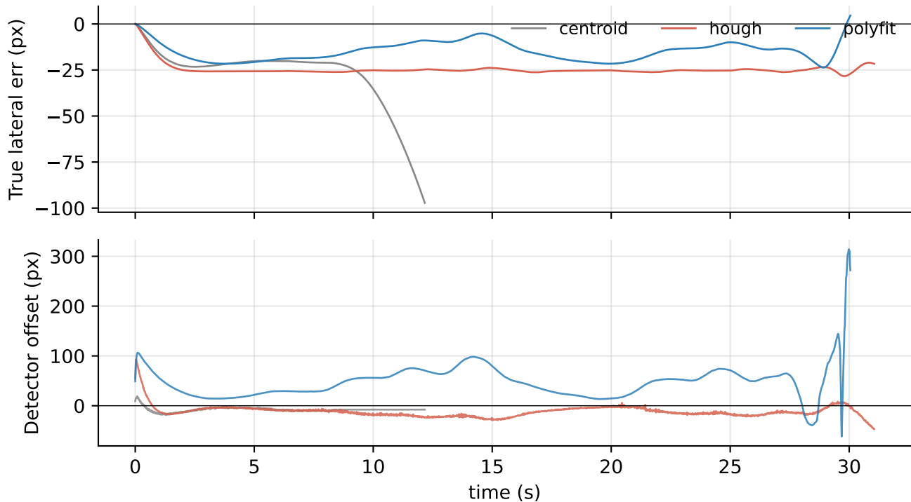
Snake track: true vs detected lateral error (PID controller)
