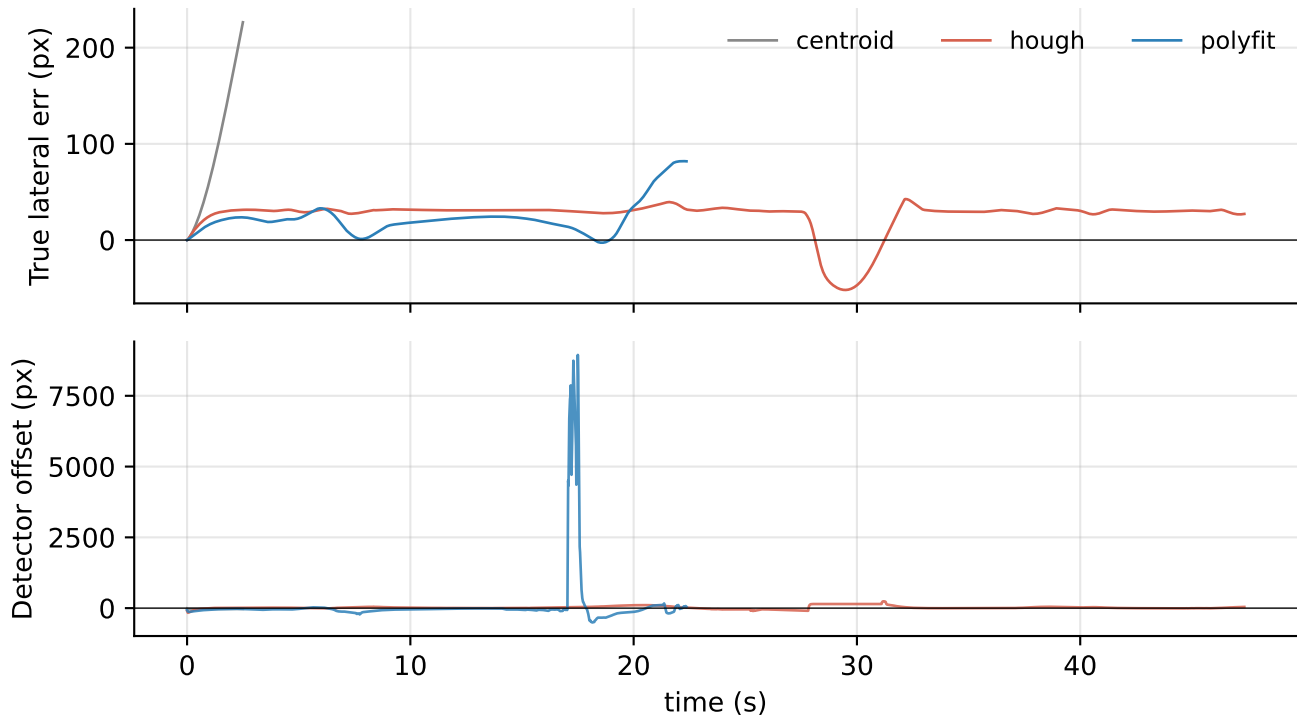
Red Bull Ring: true vs detected lateral error (PID controller)
