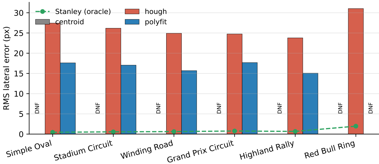
Lateral RMS error per track (PID controller)
