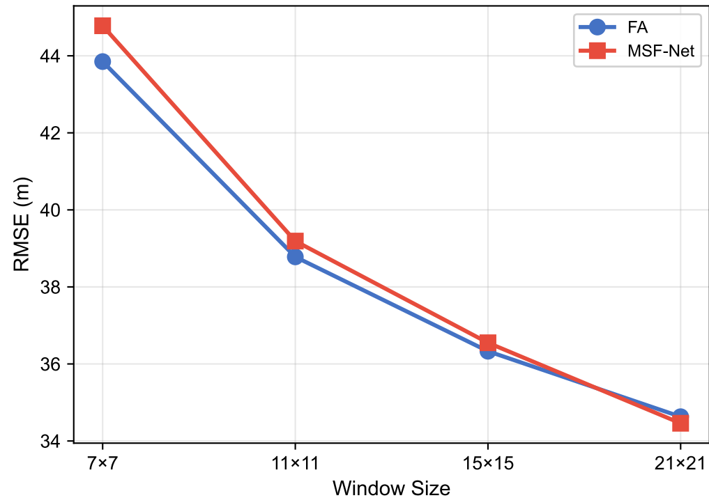
(a) RMSE vs Window Size
