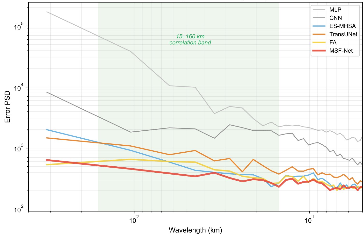
Radially Averaged Error PSD (Xisha)
