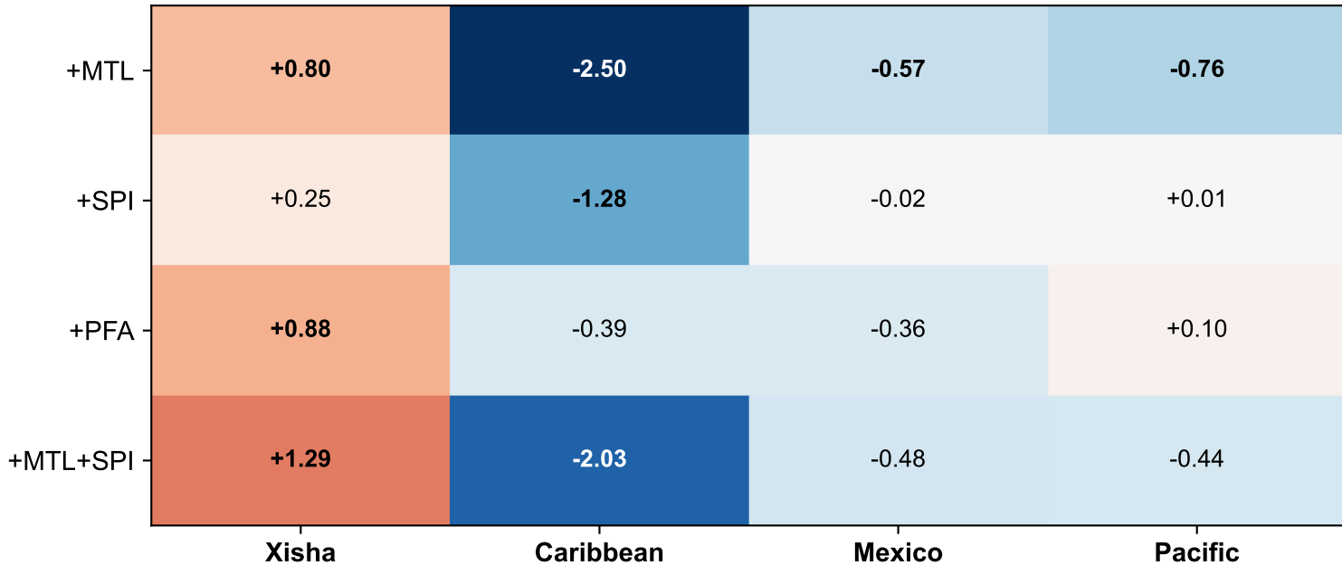
Implicit Physics: RMSE Change vs Baseline
