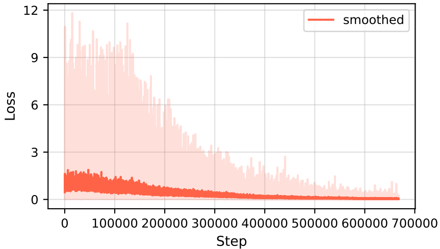
Rotation Loss
