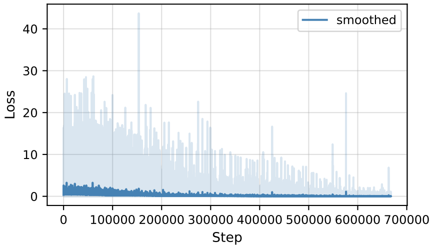
Translation Loss
