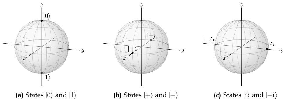
Figure 2.4: Bloch Sphere [wong2022introduction]
