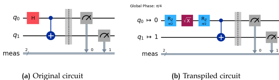
Figure 4.2: Transpilation example
