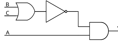
(c) Corresponding circuit
