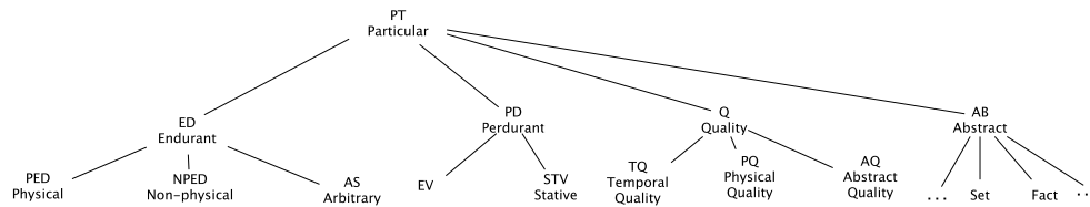
Figure 3.3: First layer of DOLCE taxonomy [borgo2022dolce]
