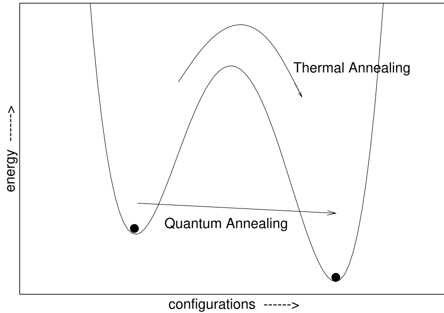
Figure 2.10: Simulated and quantum annealing [k2005transverse]
