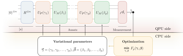
Figure 7.1: QAOA scheme [blekos2024review]
