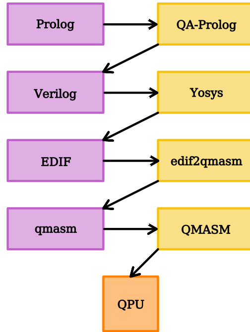
Figure 5.1: QA-Prolog pipeline
