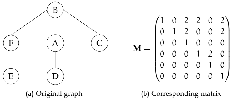
Figure 4.4: Ising formulation
