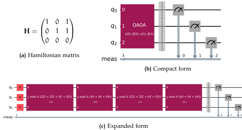
Figure 7.2: QAOA circuit
