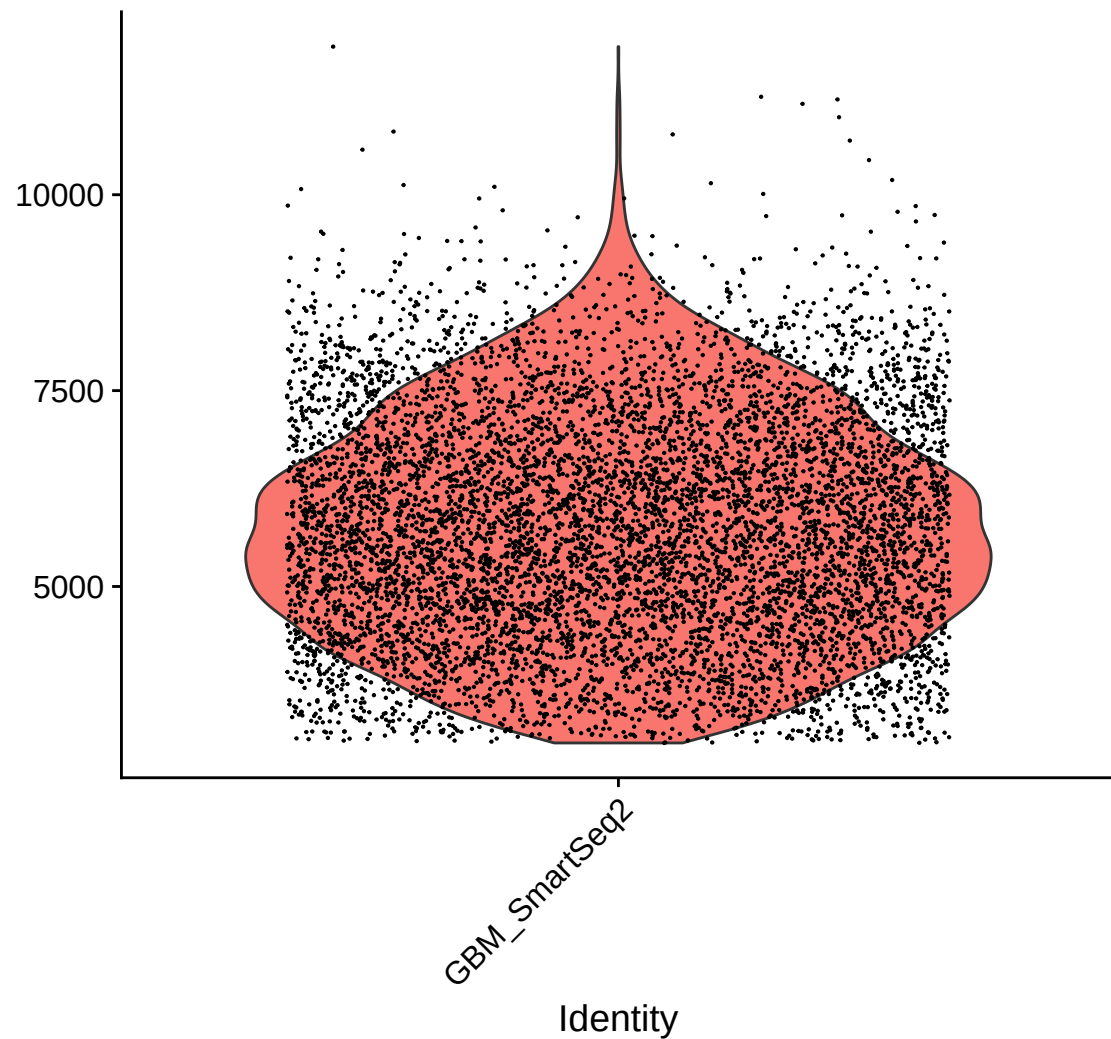
nFeature_RNA
