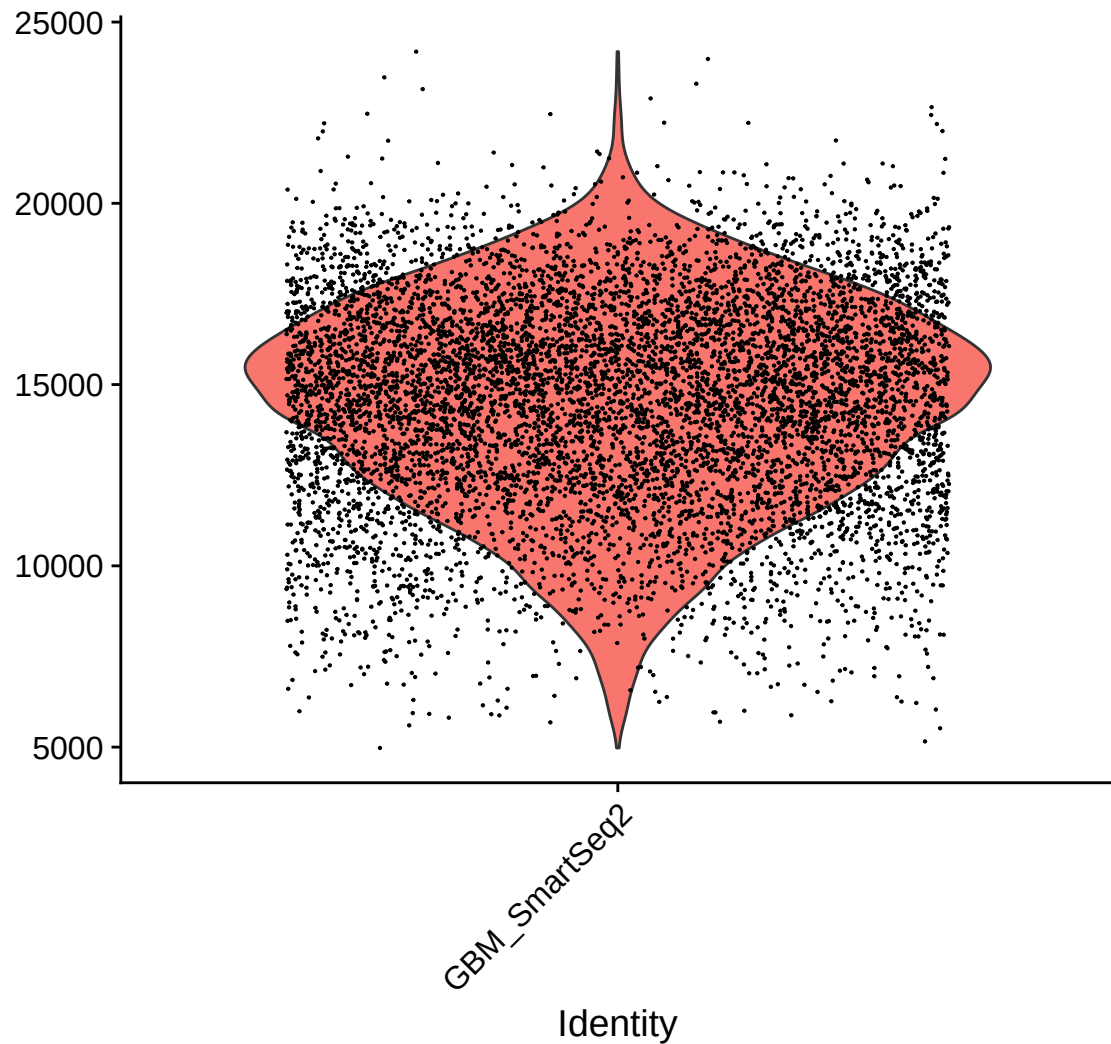
nCount_RNA
