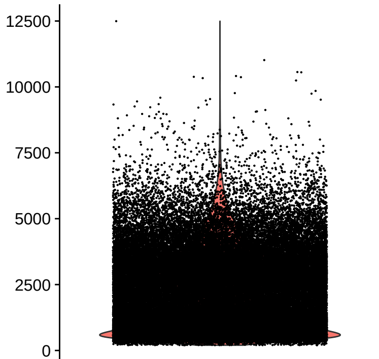
nFeature_RNA
