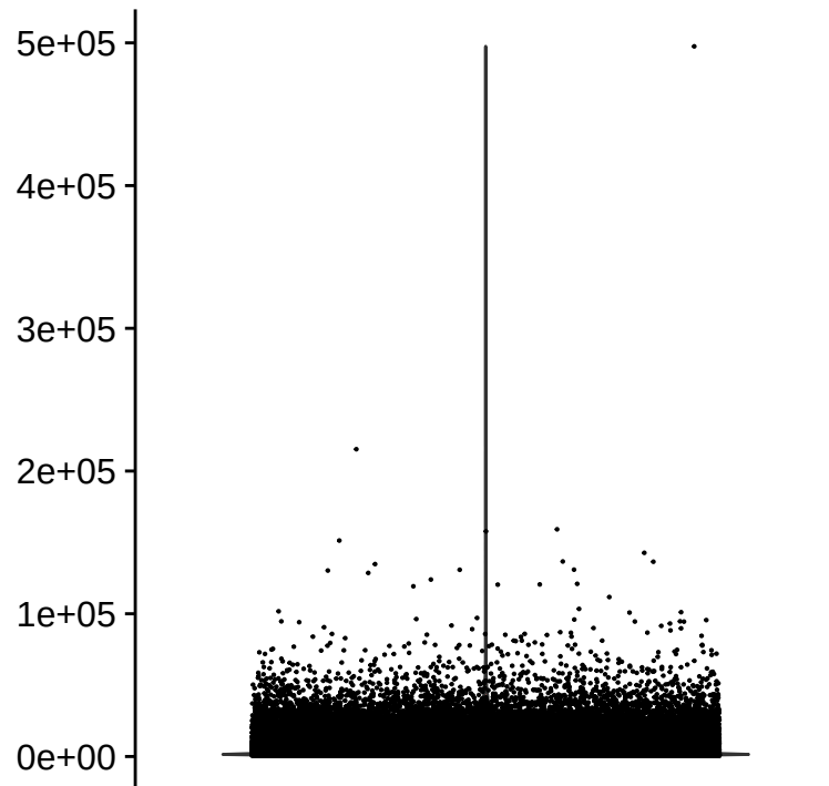
nCount_RNA
