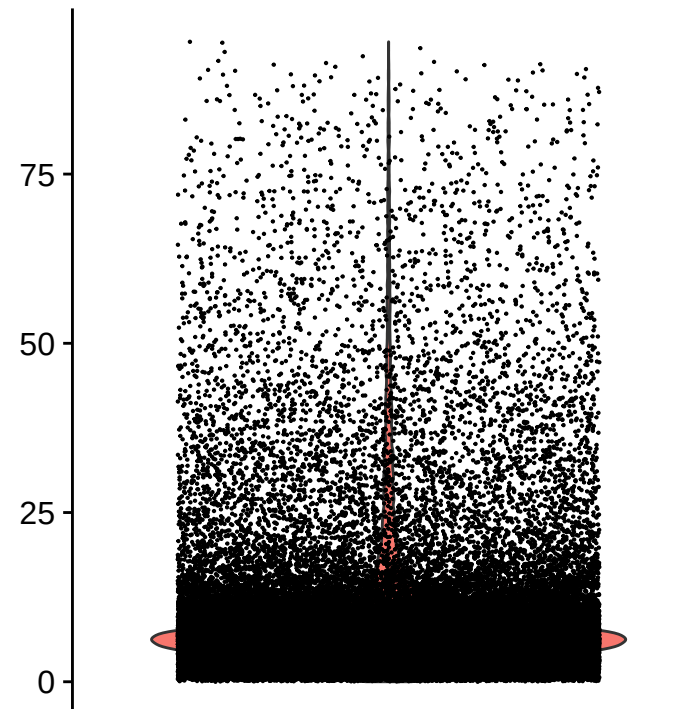
percent.mt
