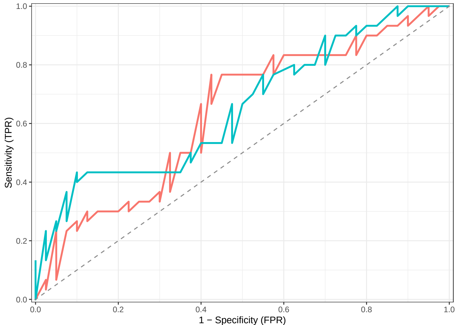
Univariate ROC: RP vs SD_PD (BestResponse_2v3_4)
