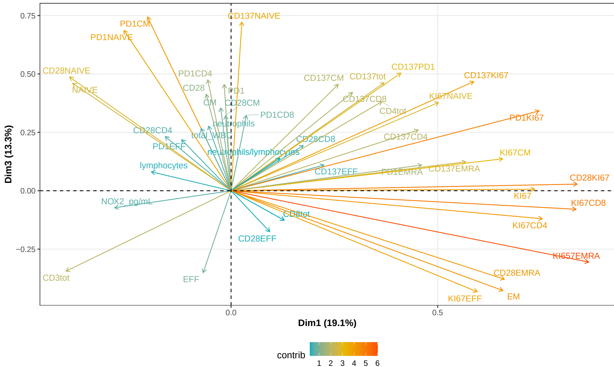
Marker Contribution Matrix (PC1 vs PC3)
