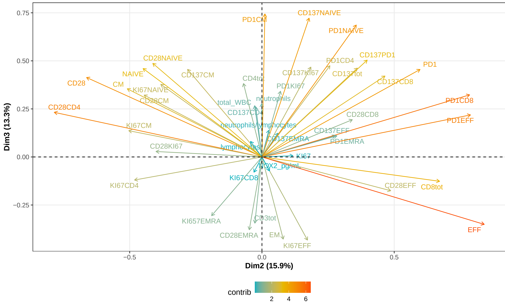
Marker Contribution Matrix (PC2 vs PC3)
