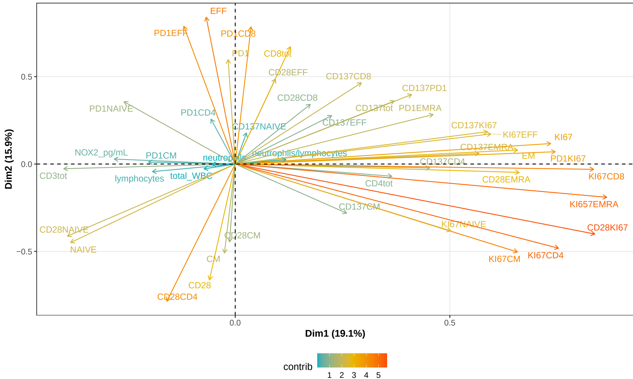
Marker Contribution Matrix (PC1 vs PC2)
