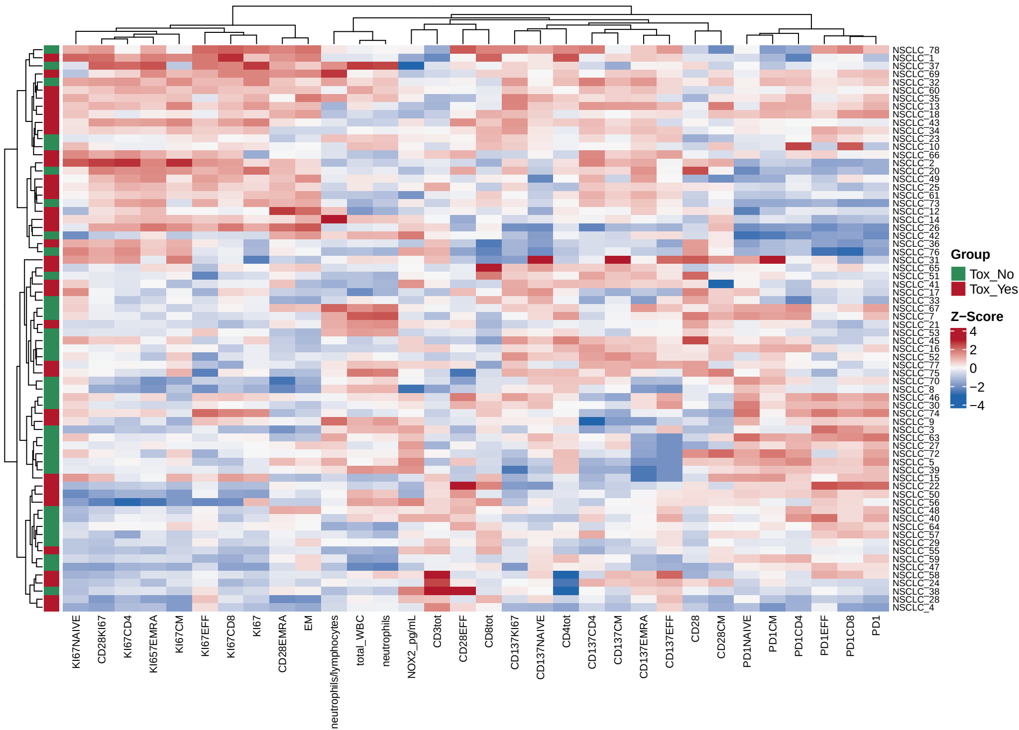
sPLS-DA Signature Heatmap
