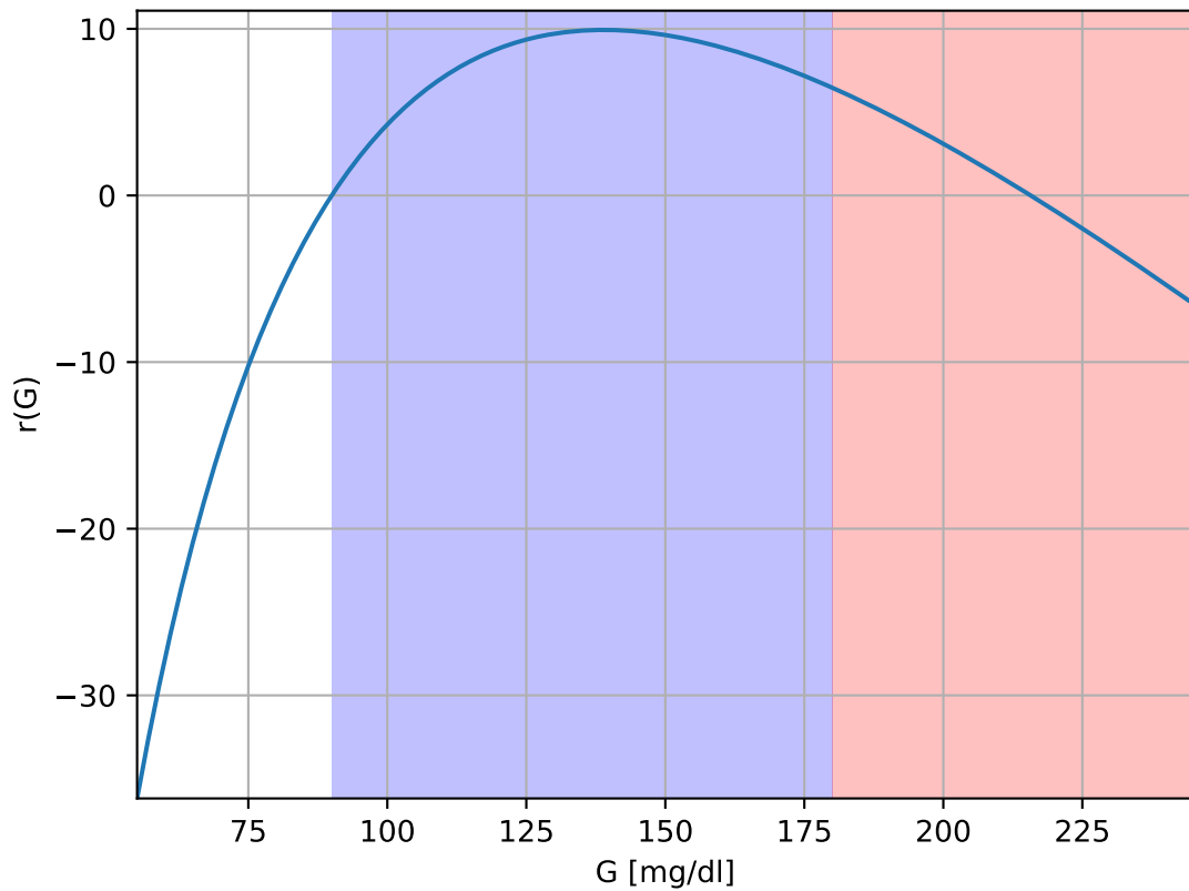
Reward Function
