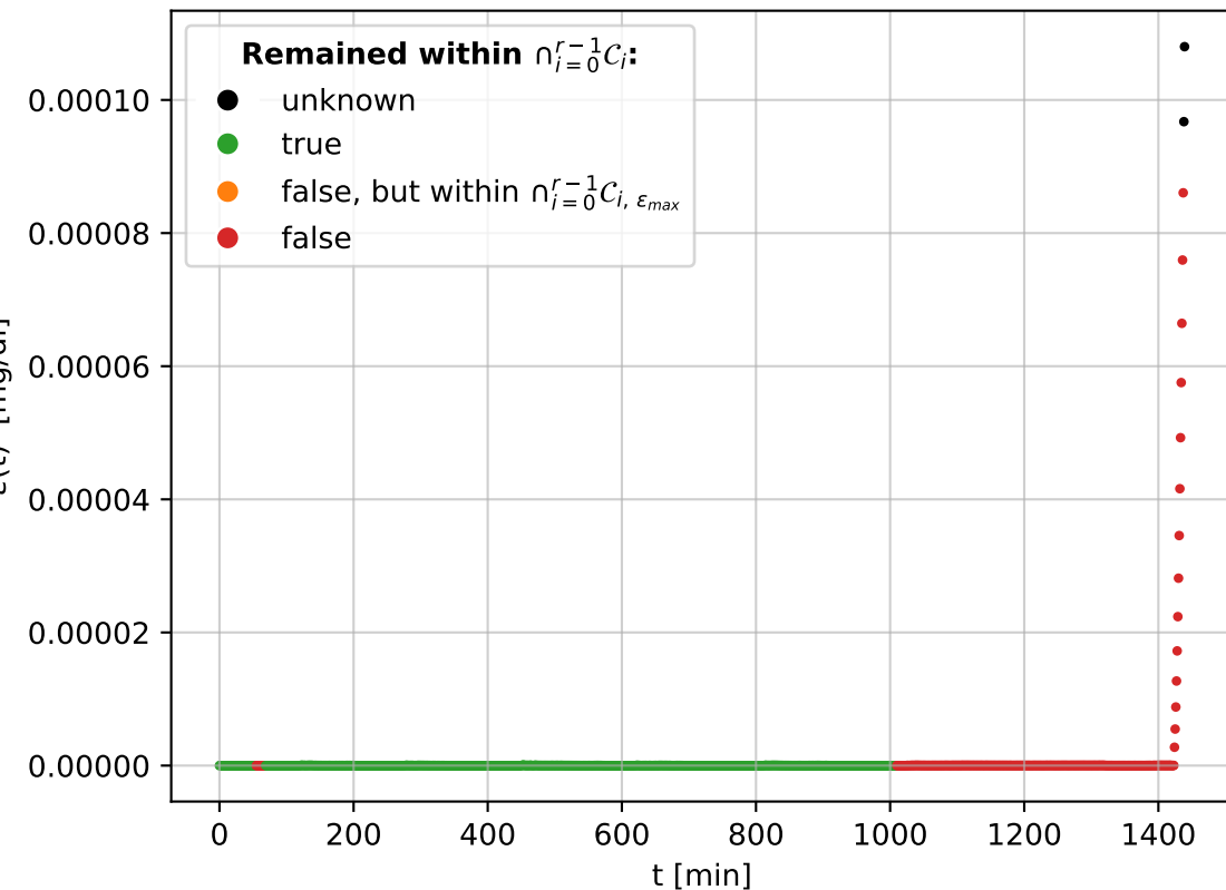
C_r Violations in an Episode Run.
