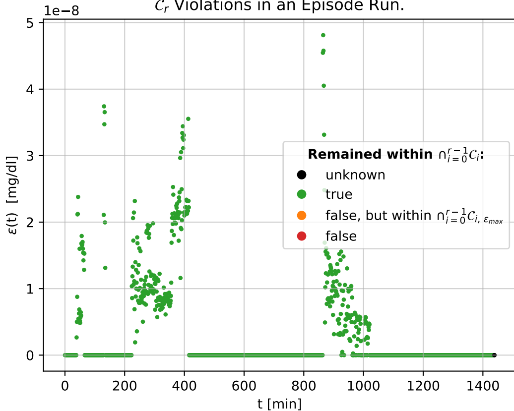
C_r Violations in an Episode Run.
