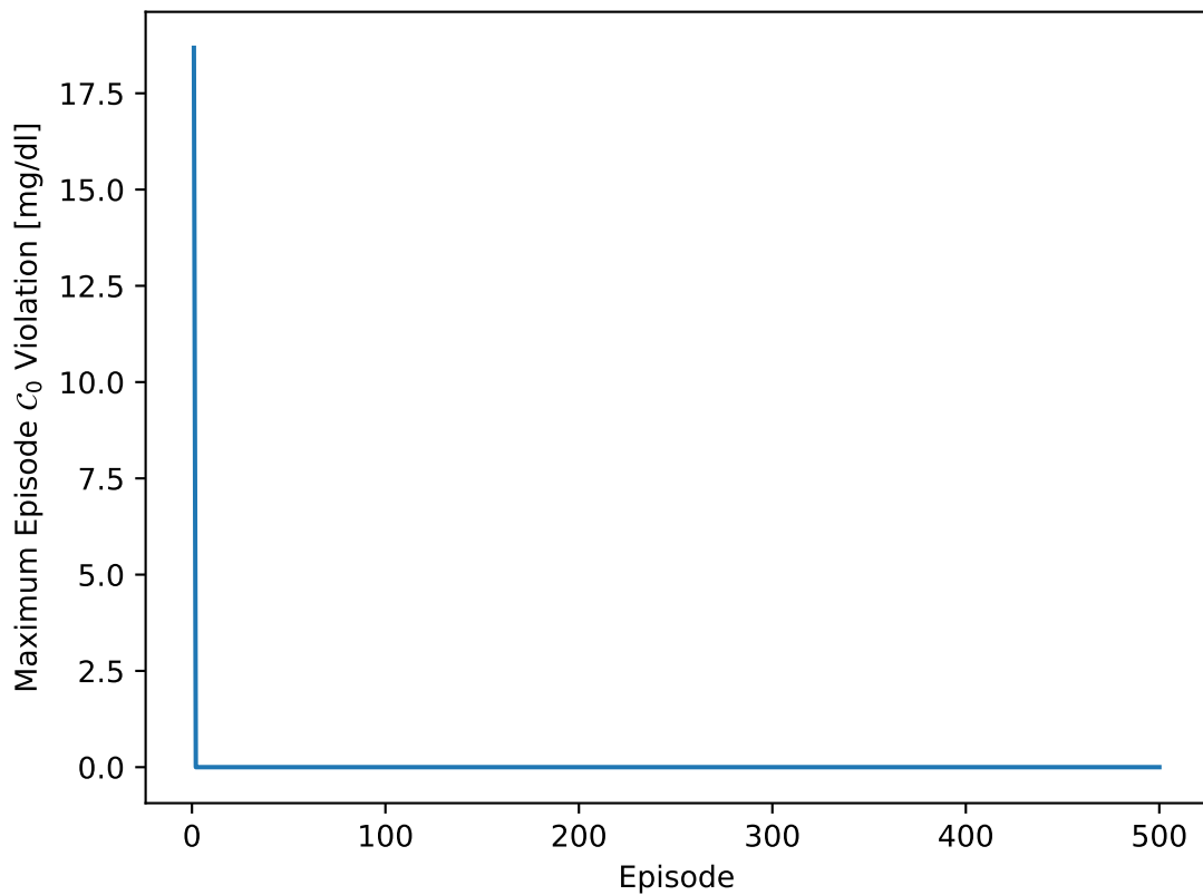
C_0 Safety Violations in Training.
