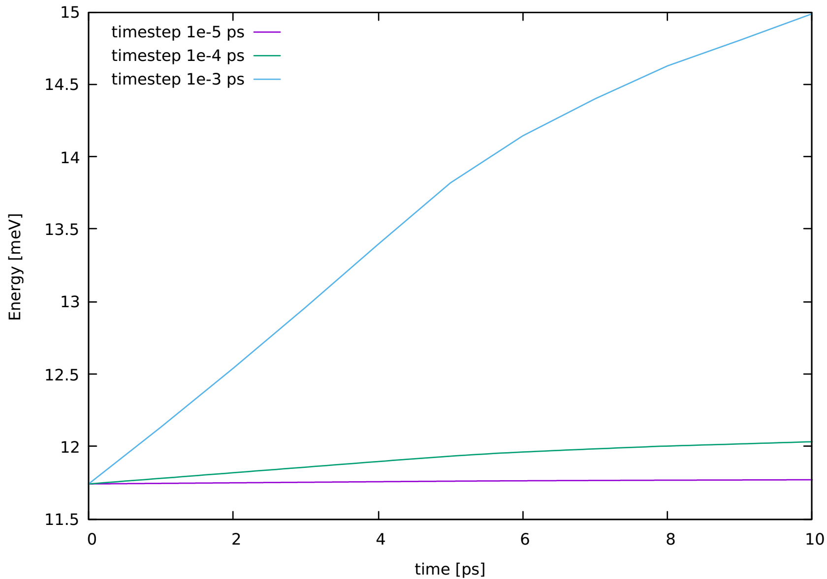
Euler integrator energy conservation, timestep comparison
