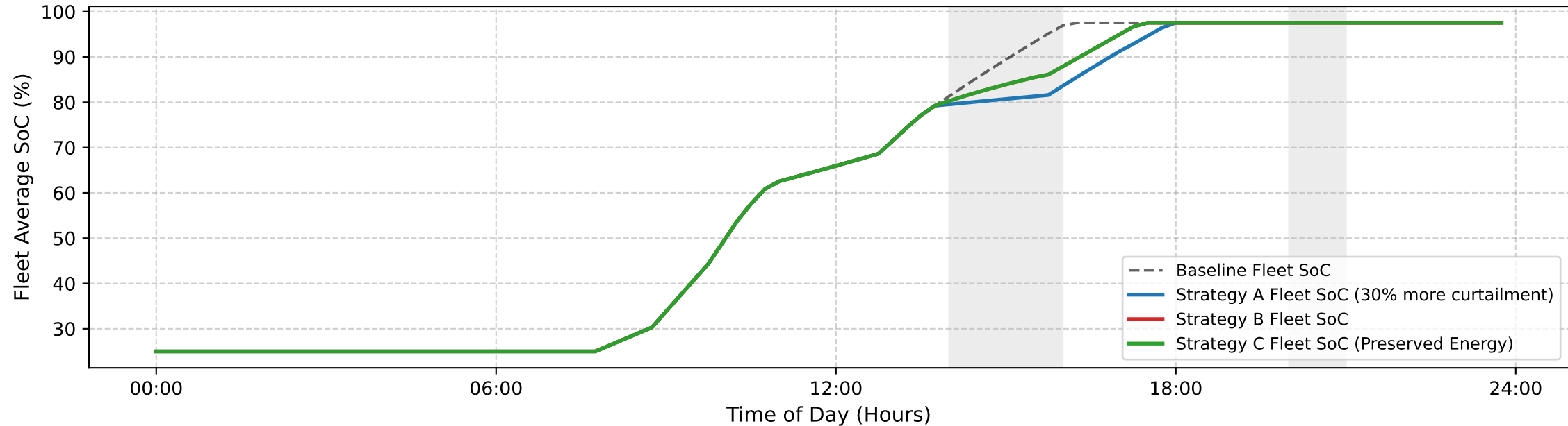
EV Fleet Average State of Charge Comparison
