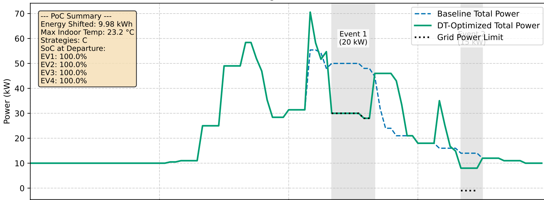
Total Building &amp; EV Power Profile
