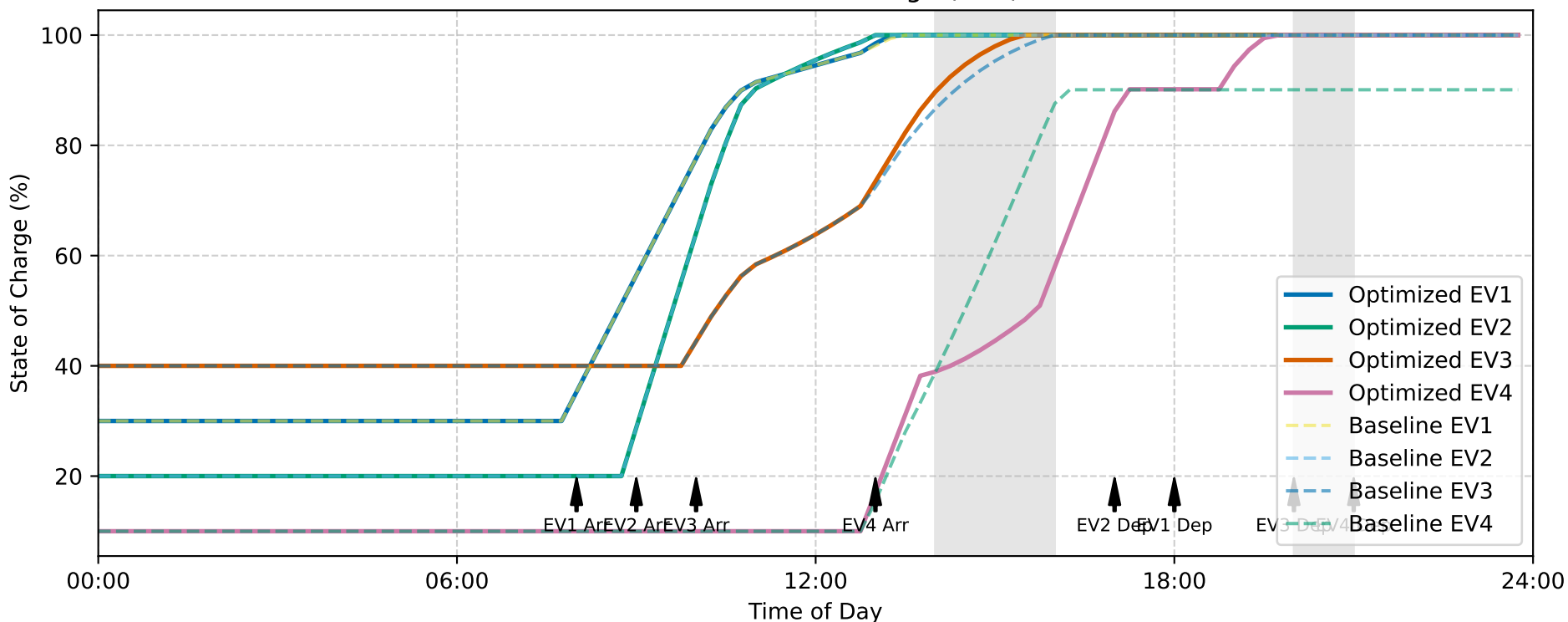
EV Fleet State of Charge (SoC)
