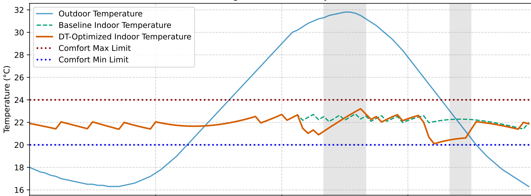
Building Indoor Thermal Dynamics
