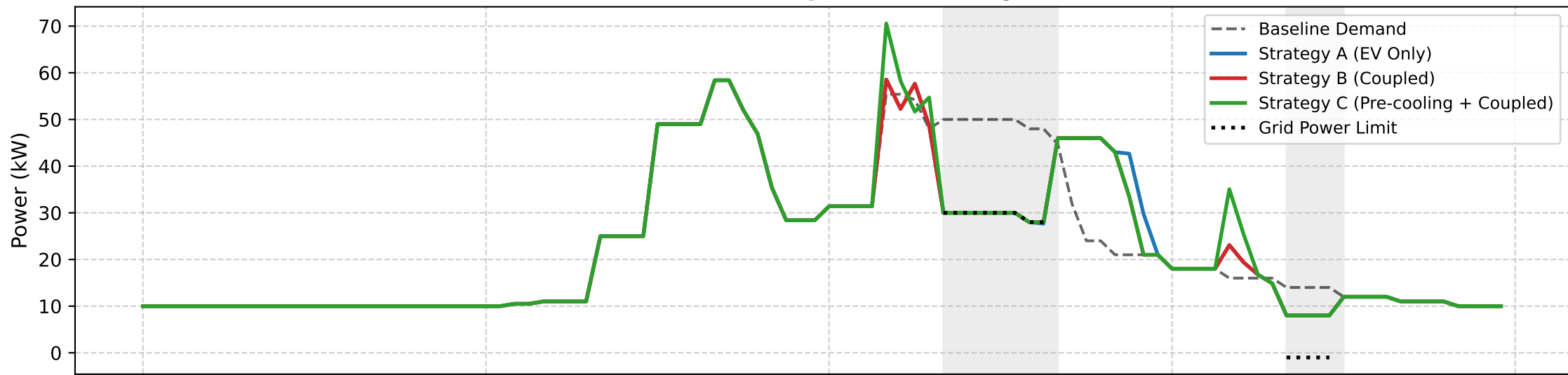
Direct Power Profile Comparison (Strategies A, B, C)
