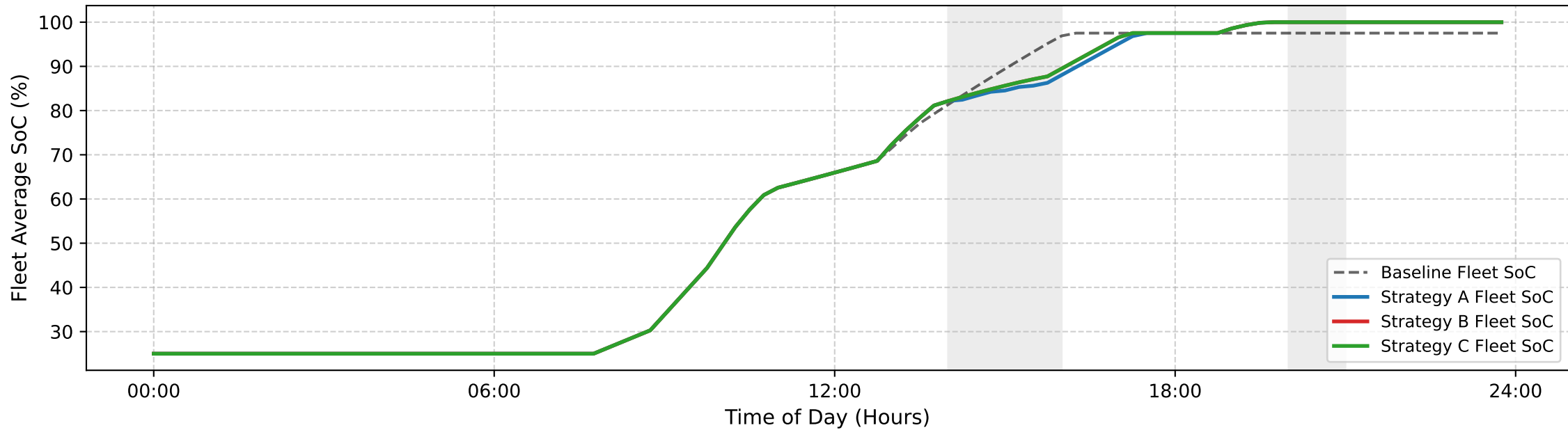
EV Fleet Average State of Charge Comparison
