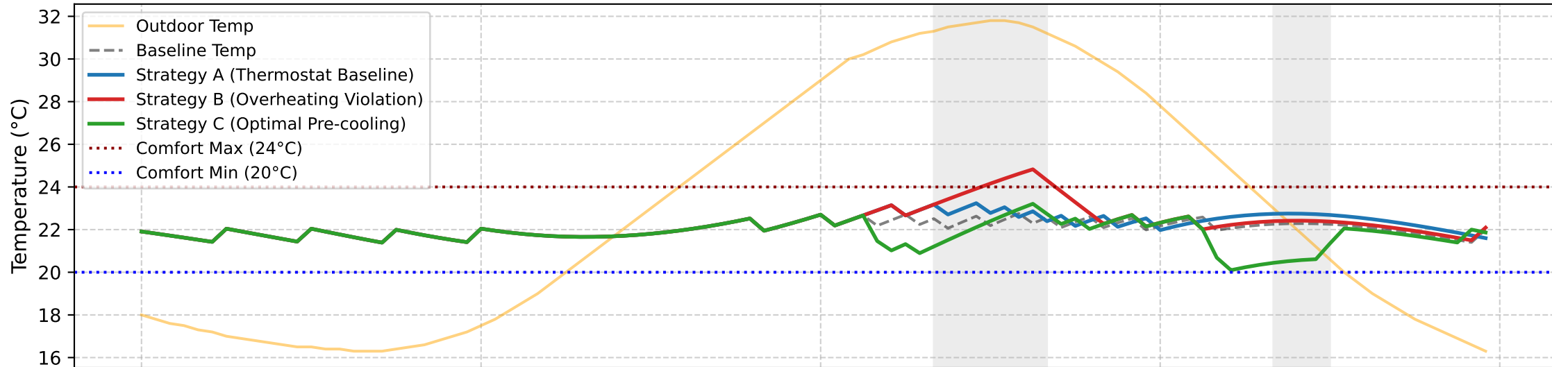
Building Thermal Dynamics Comparison
