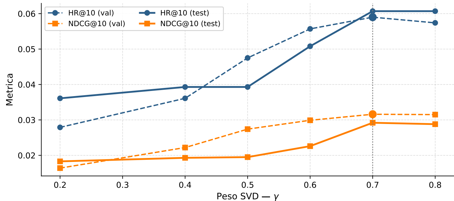
Grid search su \gamma — Hybrid PureSVD+Content-Based
