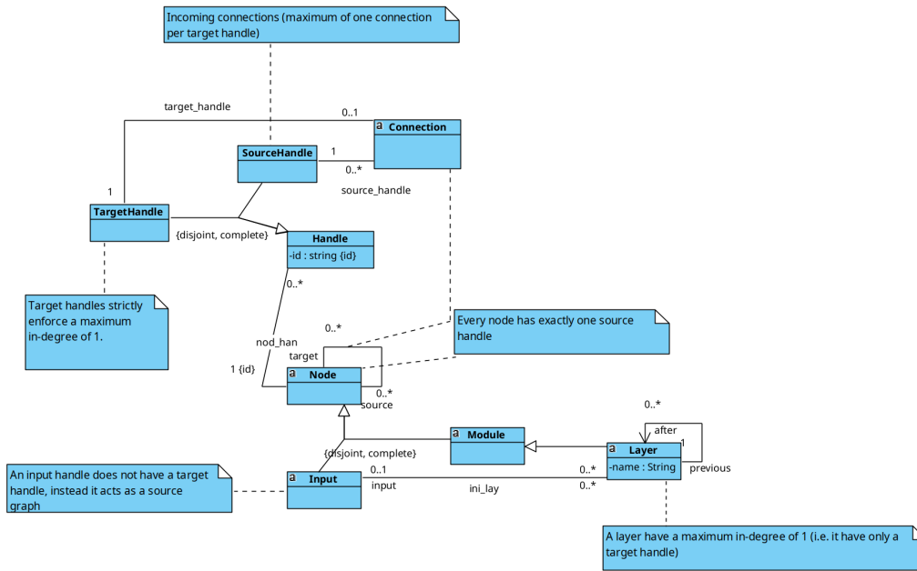
Figure 2: UML metamodel view showing the handle and connection system: SourceHandle, TargetHandle, Connection, and their association with Node.
