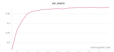
Figure 7: Validation accuracy.
