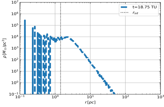
(a) Reconstructed radial stellar density profile of the remnant stellar system at t_{snap} = 18.75 , TU. The centre of the distribution was determined using the shrinking-spheres method (see, e.g., Power et al. 2003). The black dot marks the influence radius of the IMBH binary.
