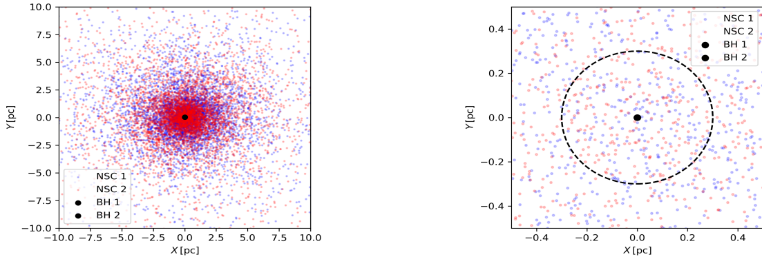
(a) Positions of the initialized NSC stars (blue and red dots) and IMBHs (black dots) in the center-of-mass frame S_{CM} at time t_{snap} = 18.75 \text{ TU} . (b) Zoom-in on the IMBH binary shown in Figure 3.9a. The dashed circle marks the KETJU regularized region at time t_{snap} = 18.75 \text{ TU} .
