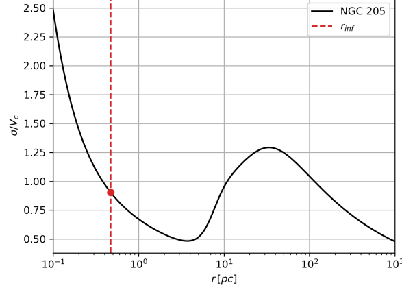
Figure 2.8: NGC 205 velocity dispersion profile (black solid line), normalized to the circular speed V_c = \sqrt{GM(r)}/r . The red vertical line marks the binary influence radius r_{inf} .
