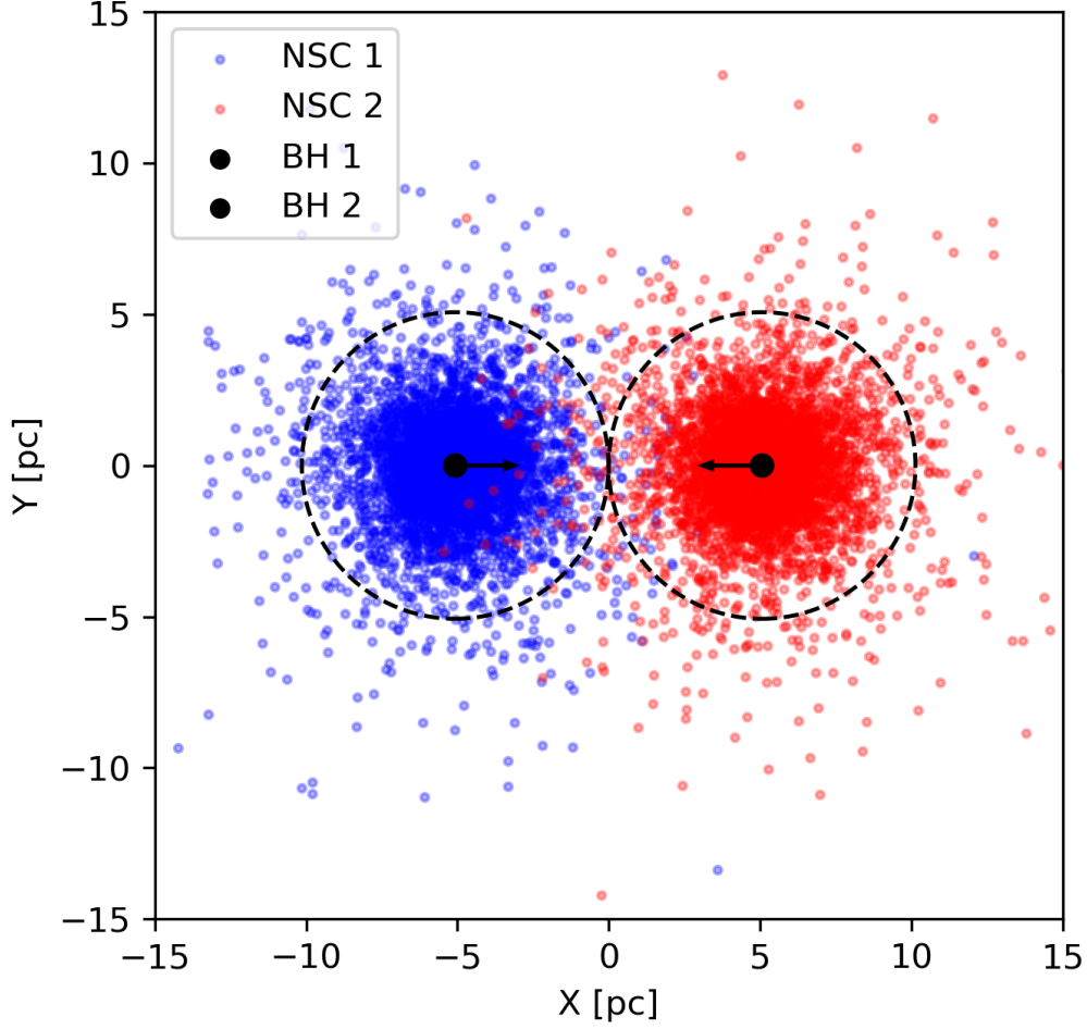
Figure 3.6: Positions of the initialized NSC stars (blue and red dots) and IMBHs (black dots) in the center-of-mass frame S_{CM} . The black arrows indicate the initial bulk velocities of the two NSCs, with lengths corresponding to the displacement over their average half-mass dynamical time. The dashed circles mark the spheres containing 90% of the total mass for each NSC.
