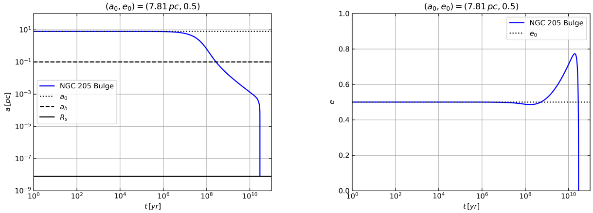
(a) NGC 205 IMBH binary semimajor axis time evolution (blue, solid line). Black horizontal lines mark the binary initial separation (dotted), hardening radius (dashed) and the binary R_s (solid).
