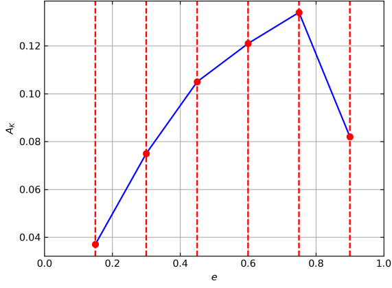
(a) Eccentricity growth rate parameter A_K (solid blue piecewise line) as a function of binary eccentricity e for binary masses ratio q = 1 . Red dashed vertical lines mark the sampled eccentricities, with red dots corresponding to the values listed in Table 2.2.
