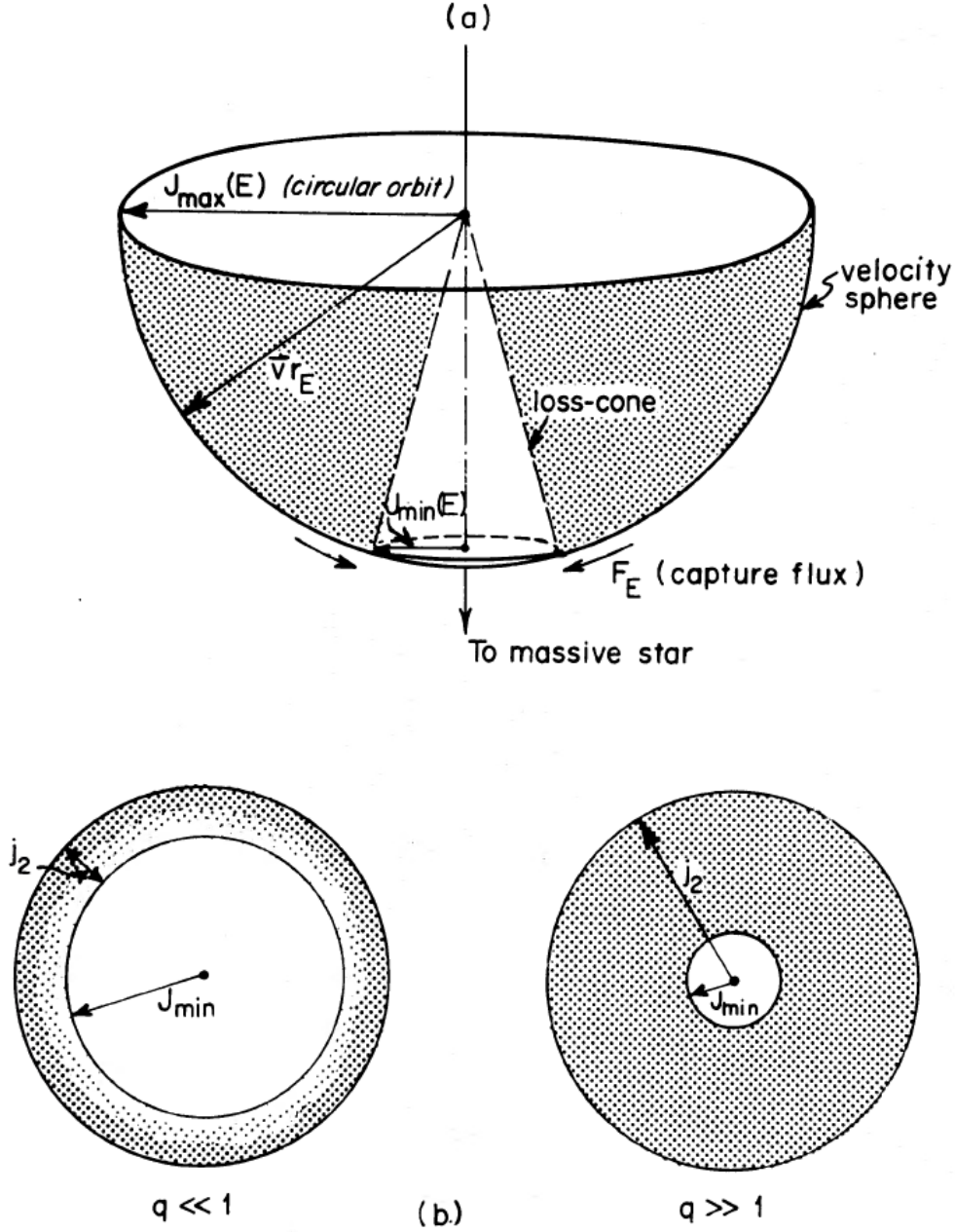
Figure 1.2: Panel (a): Velocity distribution of stars with fixed energy E_* \equiv E and angular momentum J , with the latter varying accordingly to Equation (1.67). The vertical axis points towards the compact object of mass M .
