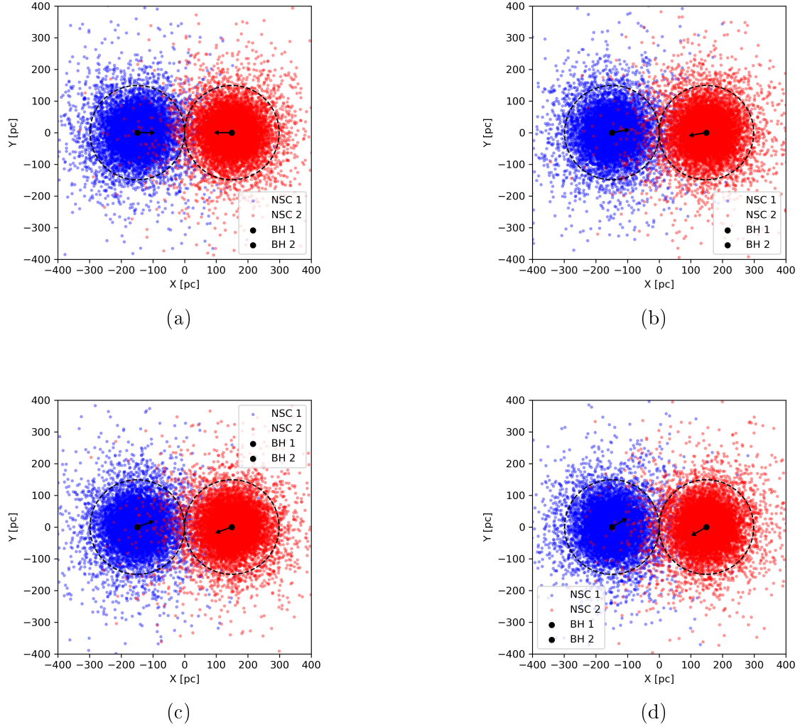
Figure 3.15: Spatial distribution of the stellar particles and IMBHs for the four initial configurations of Model 4, corresponding to different inclination angles.
