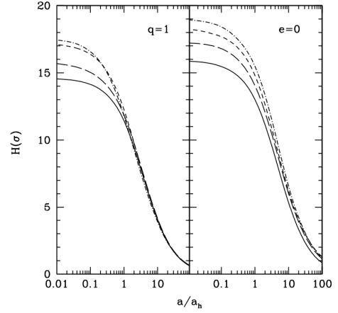
(b) Hardening rate H_u as a function of binary separation a , normalized to a_h for different eccentricities e (left) and mass ratios q (right). In both panels, solid, long-dashed, short-dashed, and dot-dashed lines correspond to e = (0, 0.3, 0.6, 0.9) and q = (1/3, 1/9, 1/27, 1/81) , respectively. Figure taken from Sesana, Haardt, et al. (2006).
