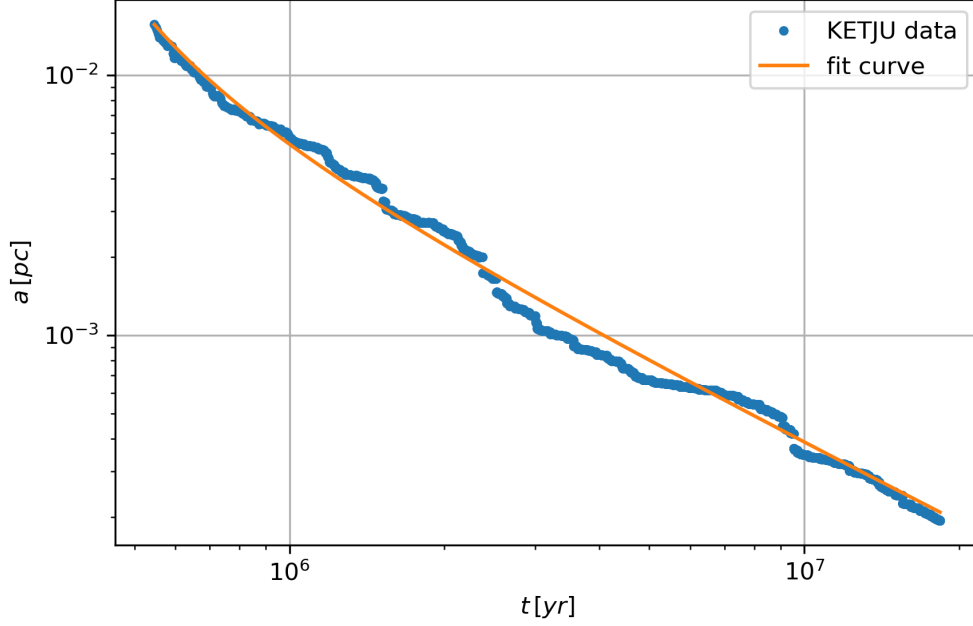
Figure 3.13: Best-fit curve (orange solid line), defined by Equation 3.34, to the KETJU output (blue dots) over the range from 0.1a_h to the IMBH binary separation at the end of the KETJU numerical simulation.
