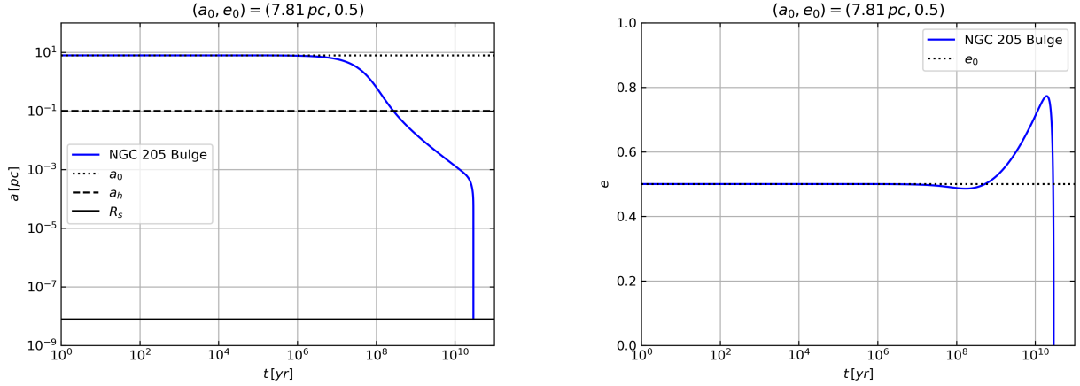
(a) NGC 205-like stellar bulge without NSC: IMBH binary semimajor-axis evolution (blue, solid line). Black horizontal lines indicate the binary initial separation (dotted), the hardening radius (dashed), and the binary R_s (solid). (b) NGC 205-like stellar bulge without NSC: IMBH binary eccentricity time evolution (blue, solid line). The black, horizontal line indicate the adopted binary initial eccentricity e_0 = 0.5 .
