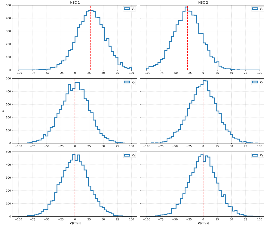
Figure 3.8: Histograms of the velocity distributions of both, N -body generated, NSCs. Each row shows the distribution of the i -th Cartesian component of the stellar velocities for NSC\ 1 (left) and NSC\ 2 (right). All histograms span [-100, 100] km/s and are divided into 50 bins, each with a width of \Delta v_i = 4 km/s. The first column distributions peak around (v_{90}, 0, 0) , while the second column around -(v_{90}, 0, 0) .
