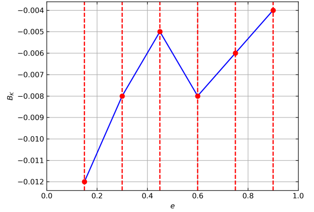
(d) Eccentricity growth rate parameter B_K (solid blue piecewise line) as a function of binary eccentricity e for binary masses ratio q = 1 . Red dashed vertical lines mark the sampled eccentricities, with red dots corresponding to the values listed in Table 2.2.
