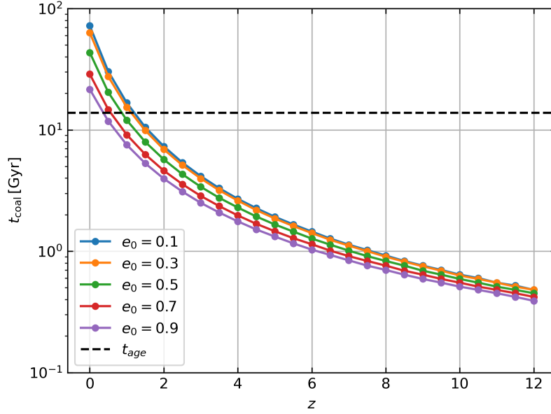
Figure 2.14: Cosmic coalescence time as a function of the redshift of IMBH binary pairing for the 125 simulations. The solid blue, orange, green, red, and violet piecewise lines connect, respectively, the points corresponding to e_0 = (0.1, 0.3, 0.5, 0.7, 0.9) across the redshift sampling. The horizontal black dashed line marks the age of the universe.
