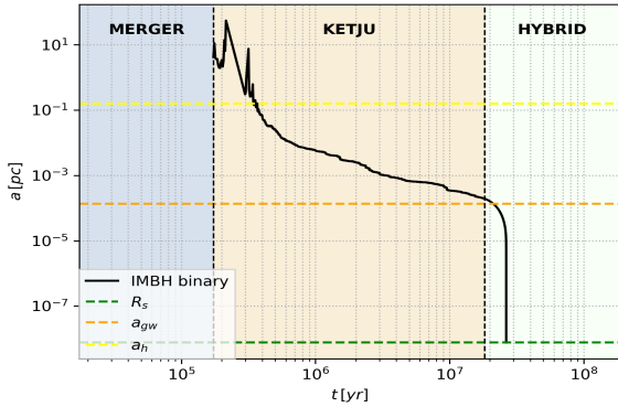
(a) IMBH binary semimajor axis time evolution.
