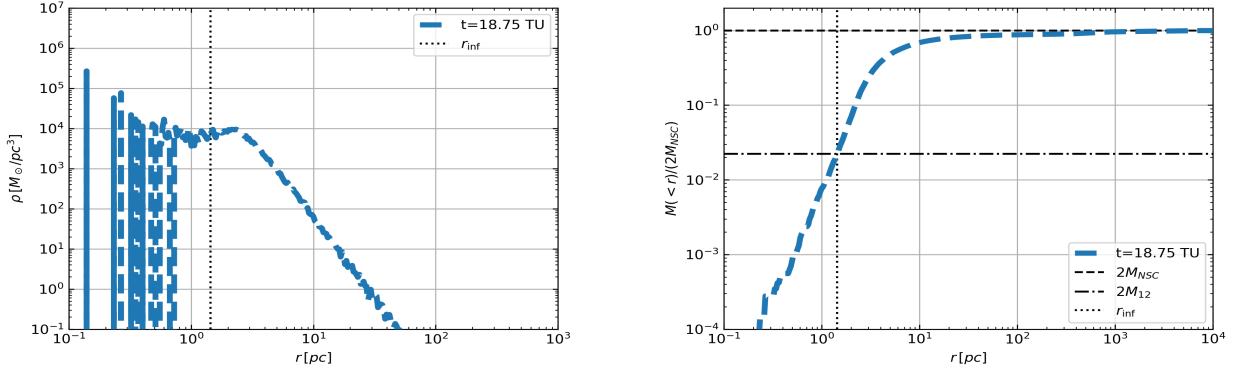
(a) Reconstructed radial stellar density profile of the remnant stellar system at t_{snap} = 18.75 TU. The centre of the distribution was determined using the shrinking-spheres method (see, e.g., Power et al. 2003). The black vertical dotted line marks the binary influence radius, r_{inf} .
