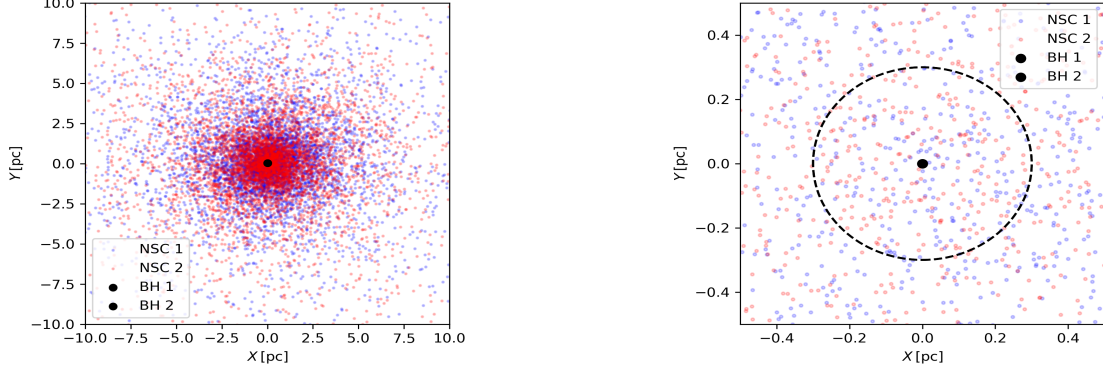
(a) Positions of the initialized NSC stars (blue and red dots) and IMBHs (black dots) in the center-of-mass frame S_{CM} at time t_{snap} = 18.75 TU.
