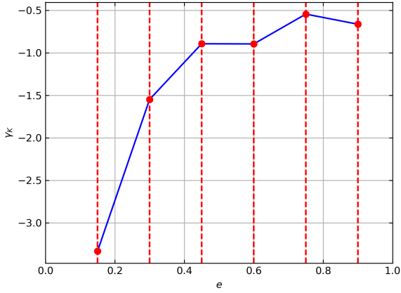
(c) Eccentricity growth rate parameter \gamma_K (solid blue piecewise line) as a function of binary eccentricity e for binary masses ratio q = 1 . Red dashed vertical lines mark the sampled eccentricities, with red dots corresponding to the values listed in Table 2.2.
