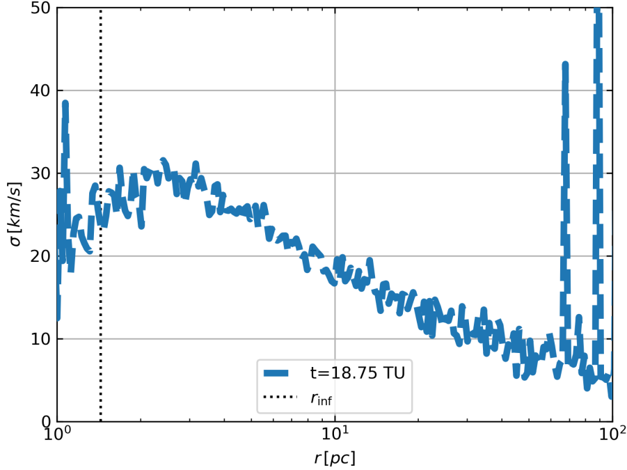
Figure 3.12: Reconstructed radial velocity dispersion profile of the remnant stellar system at t_{snap} = 18.75 \text{ TU} . The black vertical dotted line marks the binary influence radius, r_{inf} .
