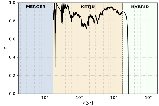
(b) IMBH binary eccentricity time evolution.
