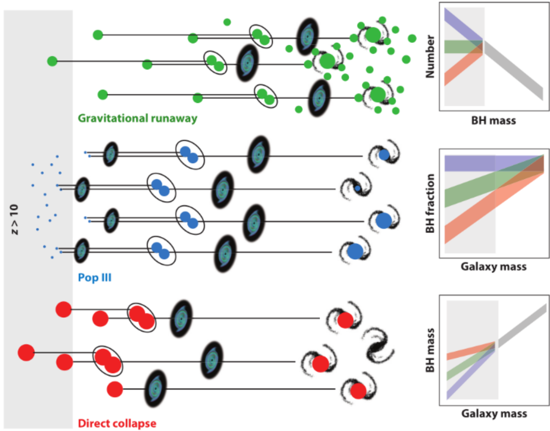
Figure 1: Schematic representation of different IMBH seeding channels, from their formation and subsequent growth through mergers and accretion to the present-day universe: Pop III stars (blue), direct collapse (red), and gravitational runaway (green). The corresponding present-day BH mass functions, occupation fractions, and BH–galaxy scaling relations are shown on the right. Figure taken from Greene et al. (2020).
