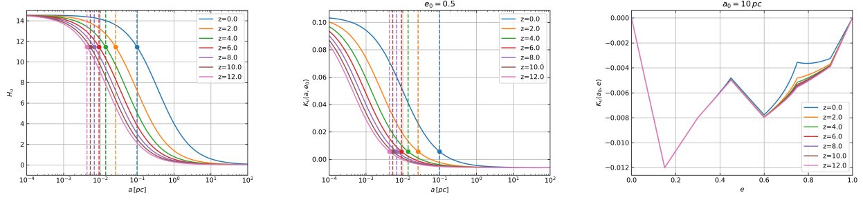
(a) Dimensionless stellar hardening rate H_u of a representative subsample of galaxy models at z = (0, 2, 4, 6, 8, 10, 12) (solid blue, orange, green, red, violet, brown, and pink lines, respectively). The corresponding hardening radii are indicated by vertical dashed lines of the same colours.
