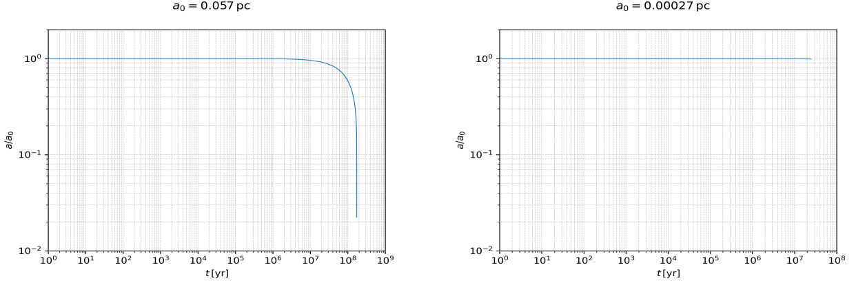
(a) Evolution of the semimajor axis of the SMBH binary with total mass M_{12} = 2 \times 10^8 M_\odot , normalized to the initial separation a_0 . The track was reconstructed from a 2-hour simulation run on a single CPU.
