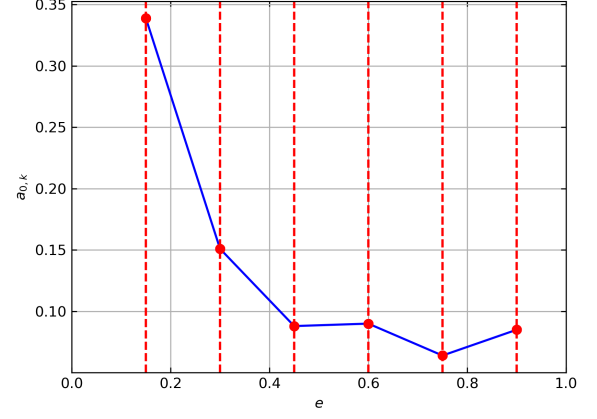
(b) Eccentricity growth rate parameter a_{0,K} (solid blue piecewise line), in a_h units, as a function of binary eccentricity e for binary masses ratio q = 1 . Red dashed vertical lines mark the sampled eccentricities, with red dots corresponding to the values listed in Table 2.2.
