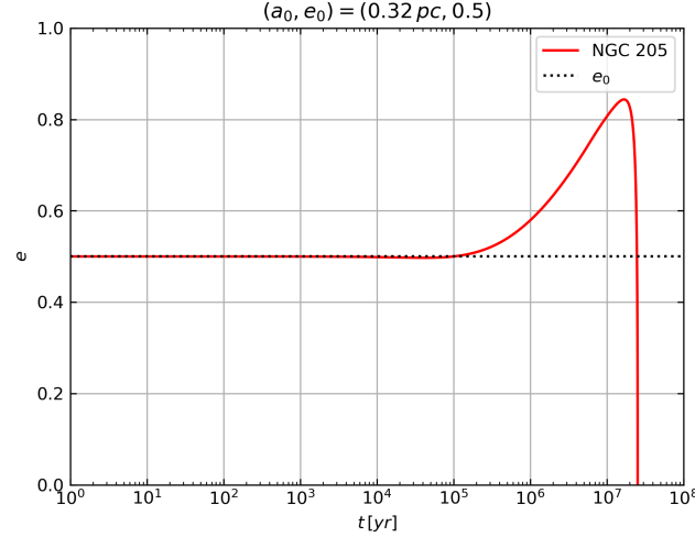
Figure 2.18: NGC 205 e vs t
