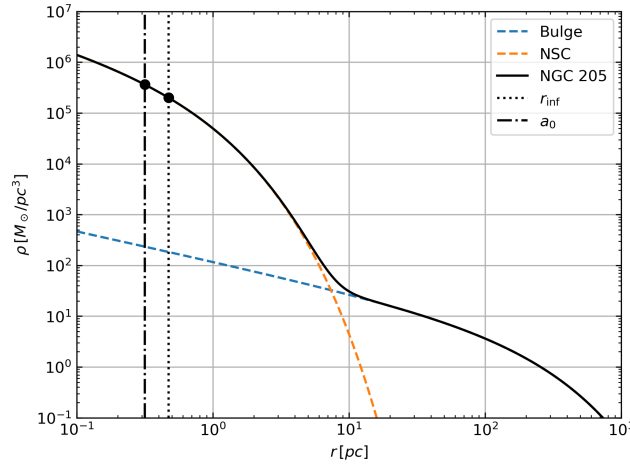
Figure 2.15: NGC 205 bulge, NSC and total mass density profile of stellar distribution.
