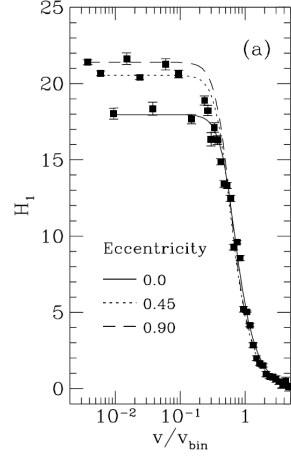
(a) "Single-velocity" binary hardening rate H_1 (see Equation 2.11) as a function of the initial stellar velocity V , normalized to the binary associated circular velocity V_{bin} = \sqrt{GM_{12}/a} , for three different values of the BH binary eccentricities, namely e = (0, 0.45, 0.90) , at fixed BH binary masses ratio q = 1 .
