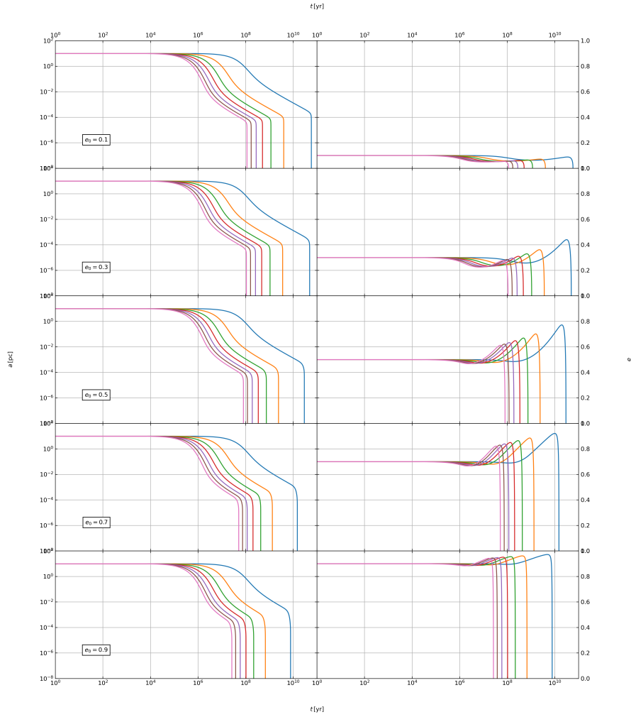
Figure 2.13: Evolutionary tracks of IMBH binaries evolving within a representative subsample of galaxy models. The left and right columns show the binary semimajor axis a(t) and eccentricity e(t) , respectively, with each pair of panels in a given row corresponding to the evolution of the same galaxy model. The five rows, from top to bottom, correspond to initial eccentricities e_0 = (0.1, 0.3, 0.5, 0.7, 0.9) , indicated by the panels on the left. Coloured curves correspond to galaxy models at z = (0, 2, 4, 6, 8, 10, 12) (blue, orange, green, red, violet, brown, and pink, respectively).
