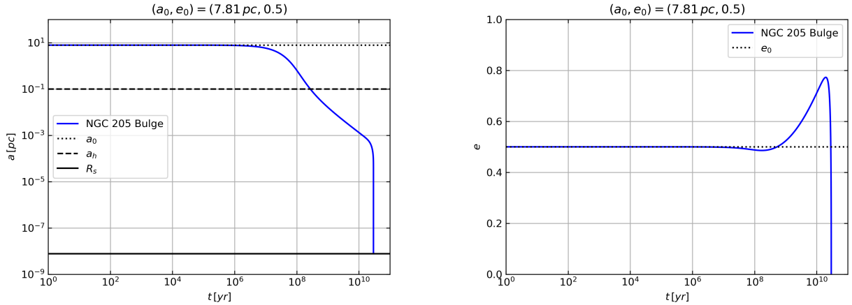
(a) NGC 205 IMBH binary semimajor axis time evolution (blue, solid line). Black horizontal lines mark the binary initial separation (dotted), hardening radius (dashed) and the binary R_s (solid). (b) NGC 205 IMBH binary eccentricity time evolution (blue, solid line). The black, horizontal line indicate the adopted binary initial eccentricity e_0 = 0.5 .
