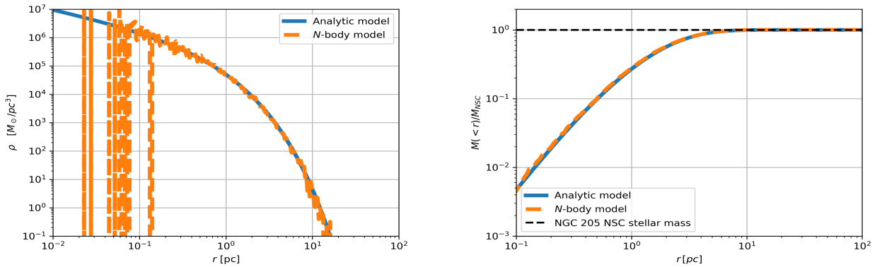
(a) Comparison between the analytic stellar mass density profile of NGC 205 NSC (blue solid line) and the corresponding profile reconstructed from the generated N -body initial conditions (orange dashed line) using Profile.dens()
