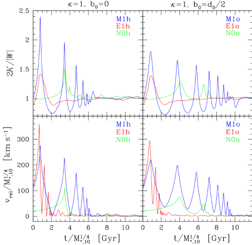
Figure 1.1: Time evolution of the virial ratio (top panels) and of the barycentric relative speed (bottom panels) for the two sets of galaxy merger simulations: head-on (left panels) and off-centre (right panels). Blue, red, and green curves refer to MOND, equivalent Newtonian, and purely baryonic Newtonian simulations, respectively. Figure taken from Carlo Nipoti et al. (2007).
