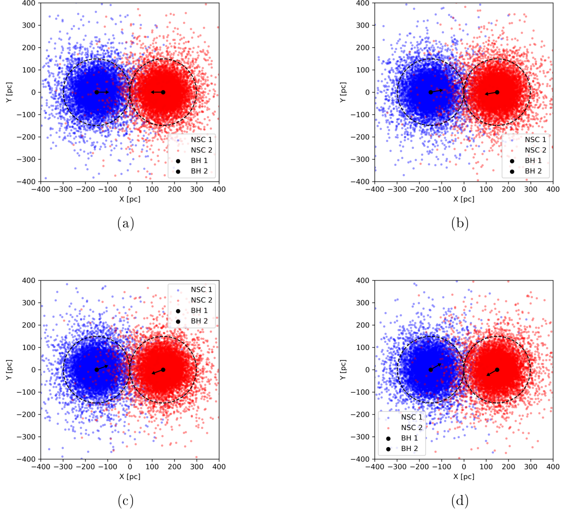
Figure 3.14: Spatial distribution of the stellar particles and IMBHs for the four initial configurations of Model 4, corresponding to different inclination angles.
