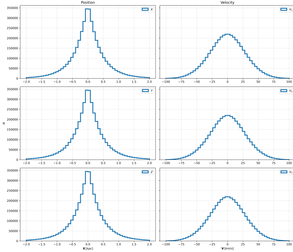
Figure 3.2: Histograms of the position and velocity distributions of the NGC 205, N -body generated, stellar components (bulge and NSC). Each row shows, on the left, the distribution of the i -th Cartesian component of the stellar positions and, on the right, the corresponding distribution of the i -th component of the stellar velocities. The position histograms span [-2, 2] \text{ kpc} and are divided into 50 bins, each with a width of \Delta x_i = 80 \text{ pc} , while the velocity histograms span [-100, 100] \text{ km/s} and are divided into 50 bins, each with a width of \Delta v_i = 4 \text{ km/s} .
