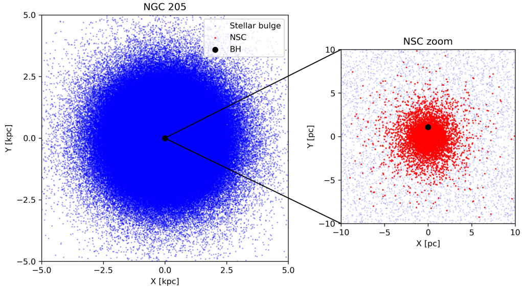
Figure 3.1: Positions of the N -body initial conditions for the NGC 205 stellar bulge, NSC, and hosted IMBH, projected onto the x - y plane. Blue and red dots represent bulge and NSC stars, respectively, while the black dot marks the IMBH. The main panel shows the system on the scale of the stellar bulge, whereas the inset provides a zoomed-in view of the NSC and IMBH.
