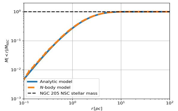
(b) Enclosed stellar mass profile.
