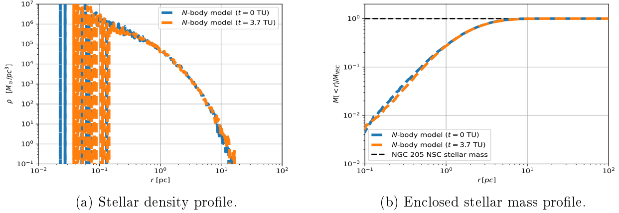
Figure 3.5: Comparison between the analytic NGC 205 stellar model and the corresponding N -body initial conditions.
