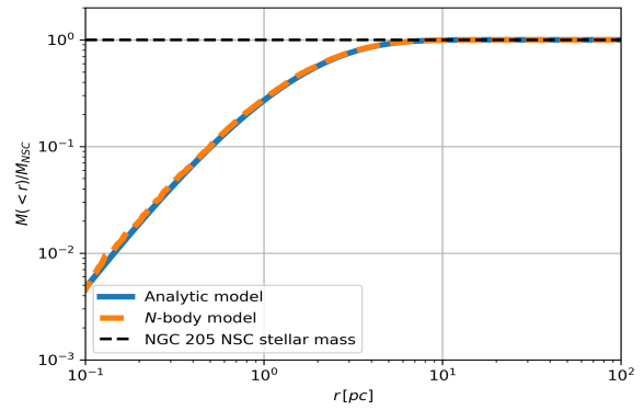
(b) Enclosed stellar mass profile.
