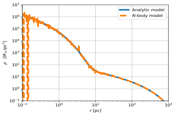
(a) Stellar density profile.
