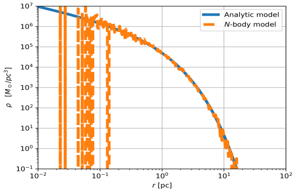
(a) Stellar density profile.
