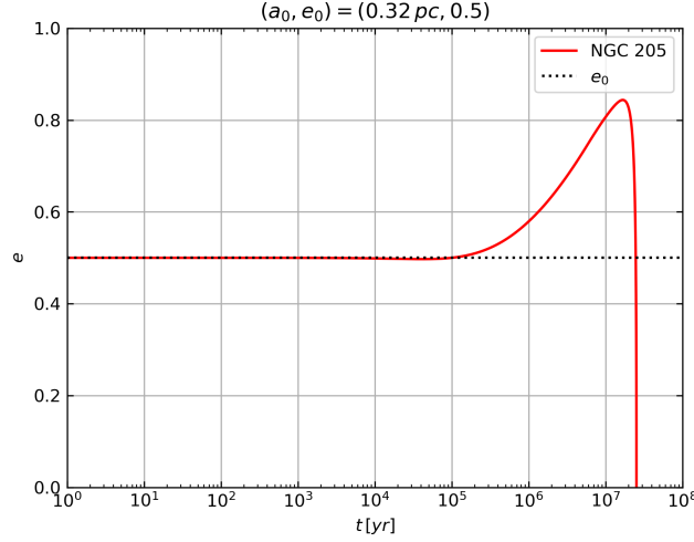
Figure 2.17: NGC 205 e vs t
