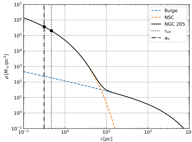
Figure 2.16: NGC 205 bulge, NSC and total mass density profile of stellar distribution.
