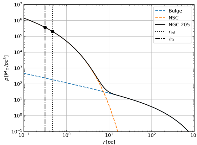
Figure 2.12: NGC 205 bulge, NSC and total mass density profile of stellar distribution.
