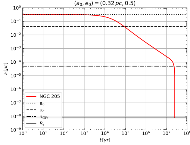
Figure 2.14: NGC 205 a vs t
