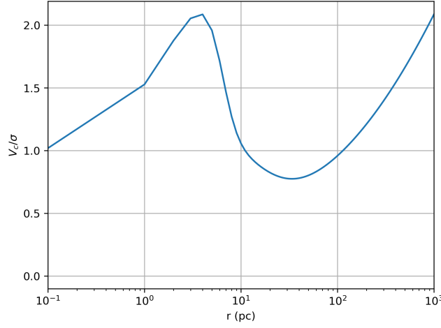
Figure 2.13: NGC 205 V_c/\sigma vs r
