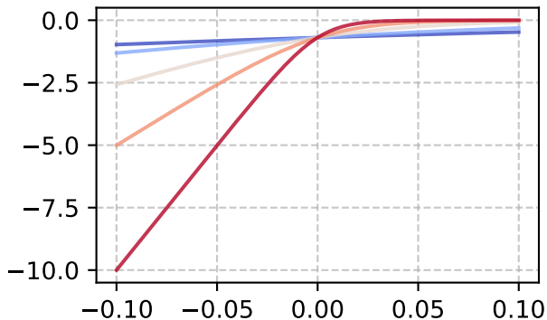
c[x = 0]
