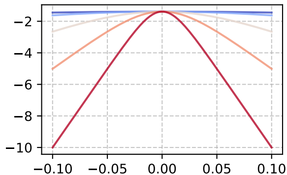
c[x = 0]
