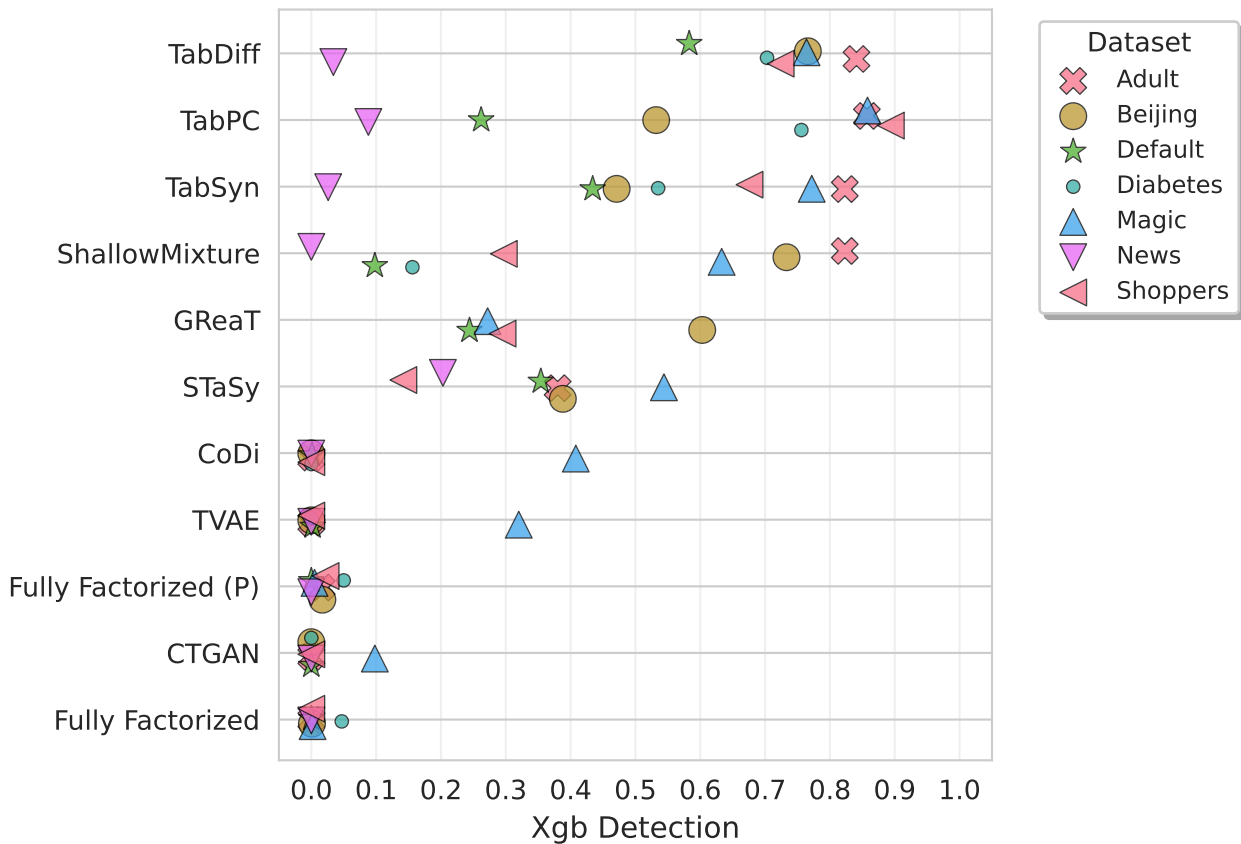
Xgb Detection by Method and Dataset
