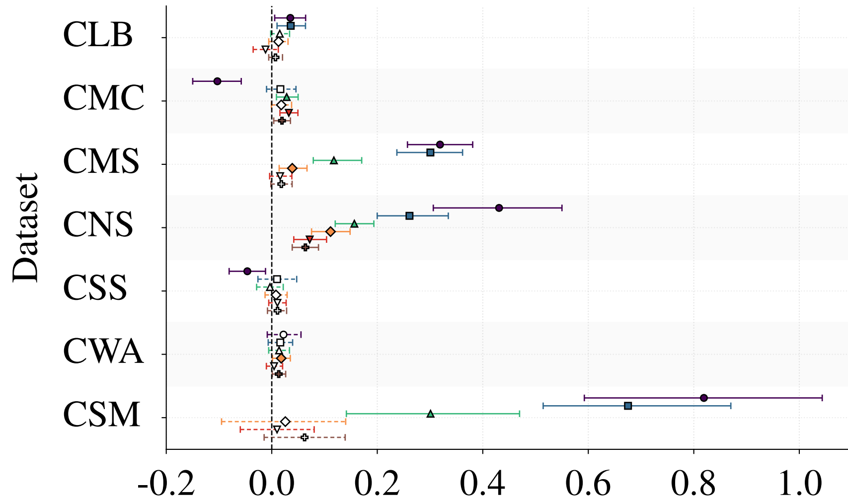
Vanilla Original vs CPDAG Minimal
