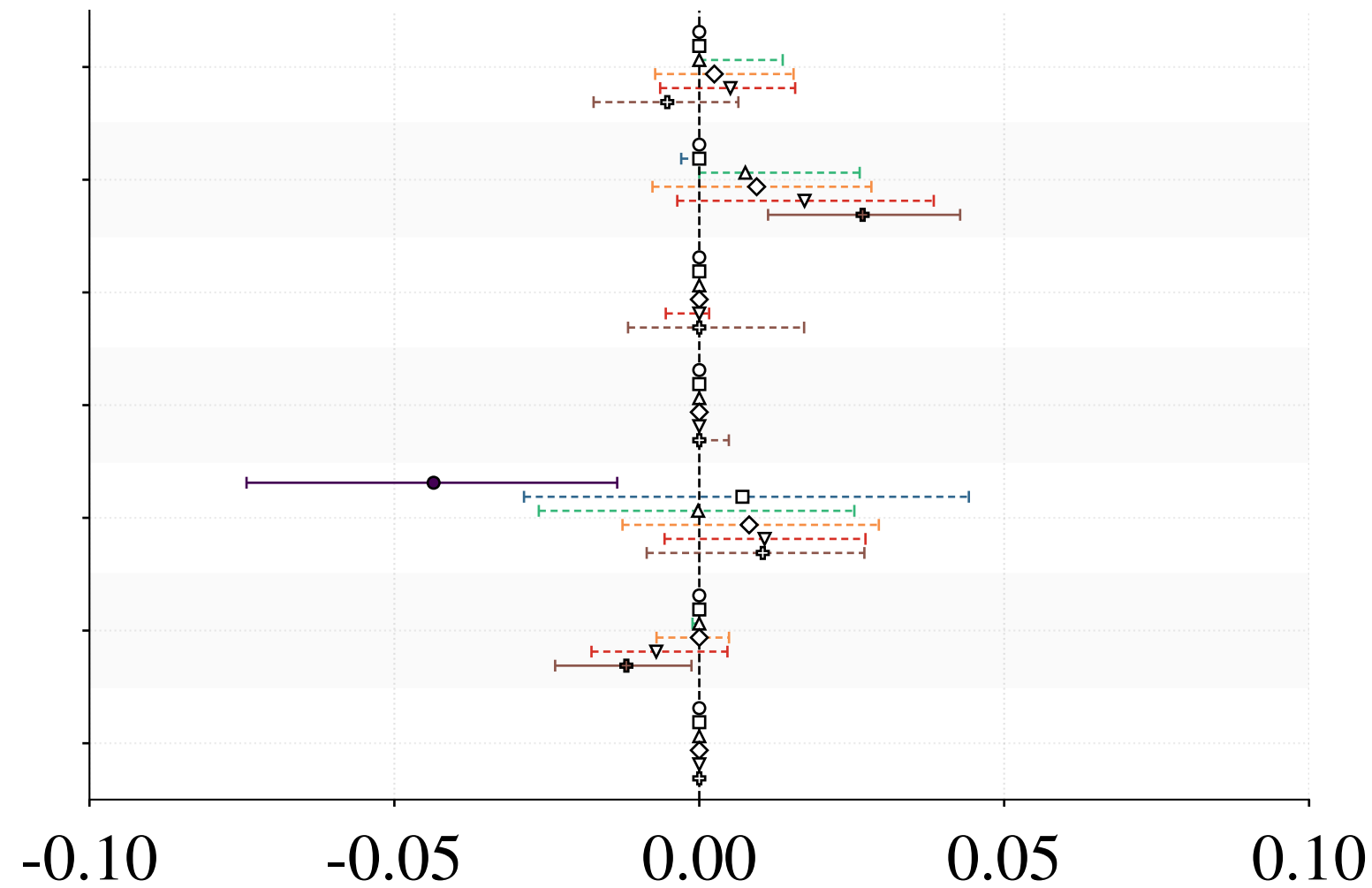
Vanilla Original vs CPDAG Discovered
