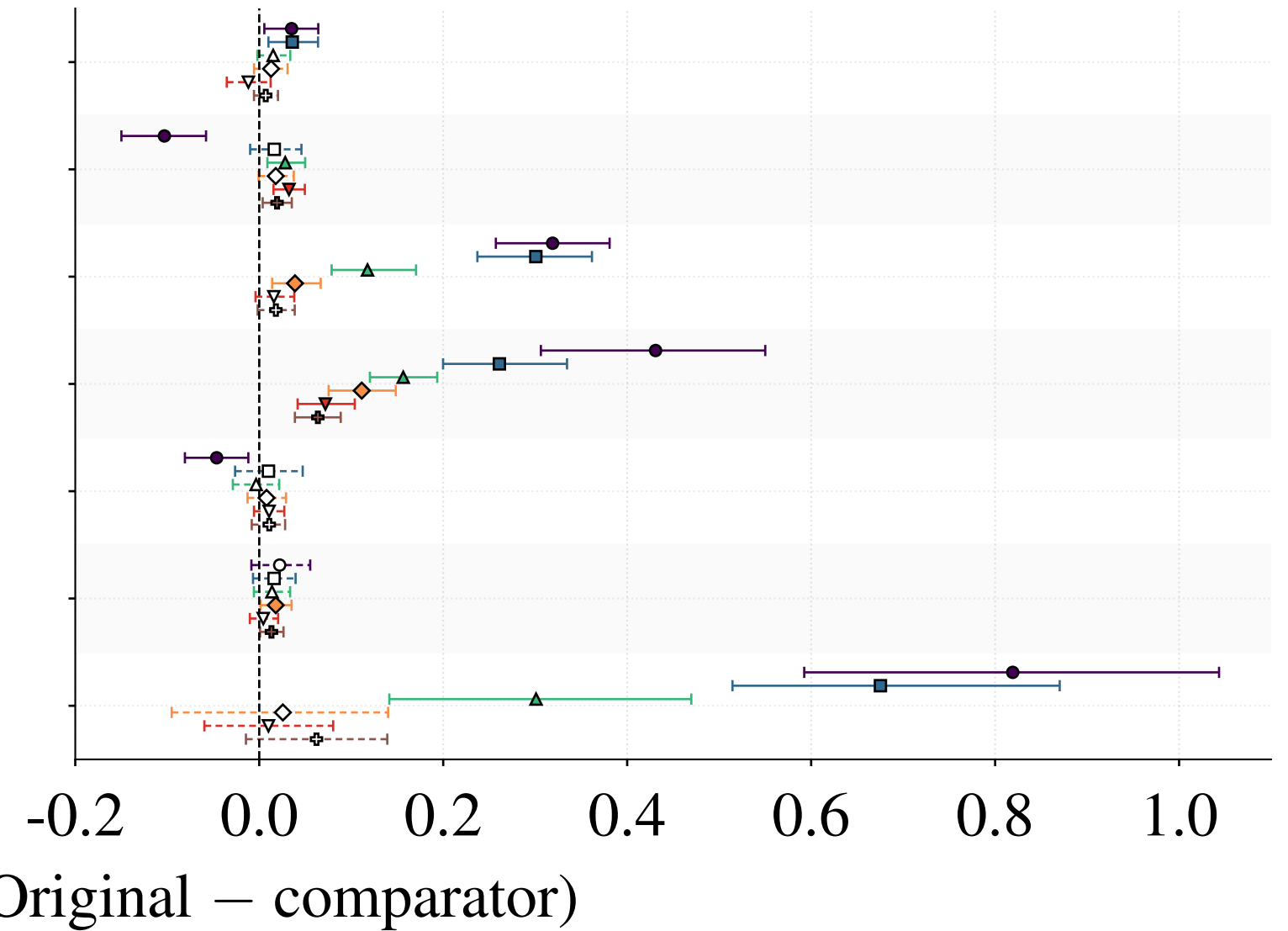
Vanilla Original vs CPDAG Minimal
