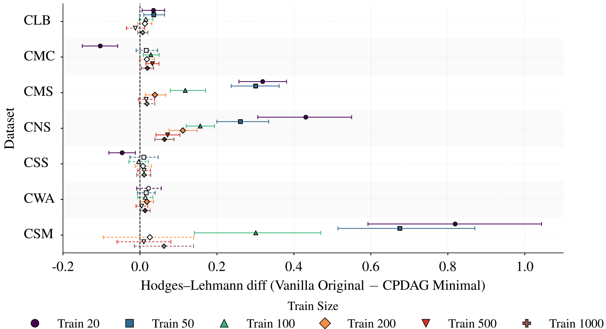
Vanilla Original vs CPDAG Minimal · ATE Difference (Estimate - Ground Truth)
