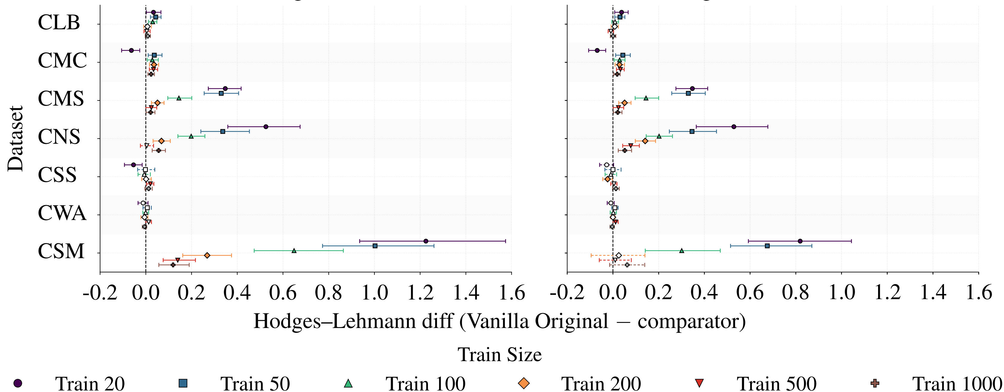
Vanilla Original vs DAG
