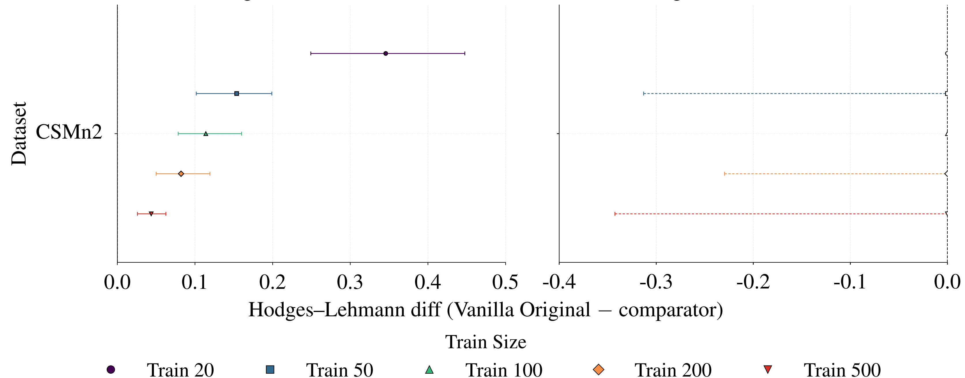
Vanilla Original vs Minimal CPDAG
