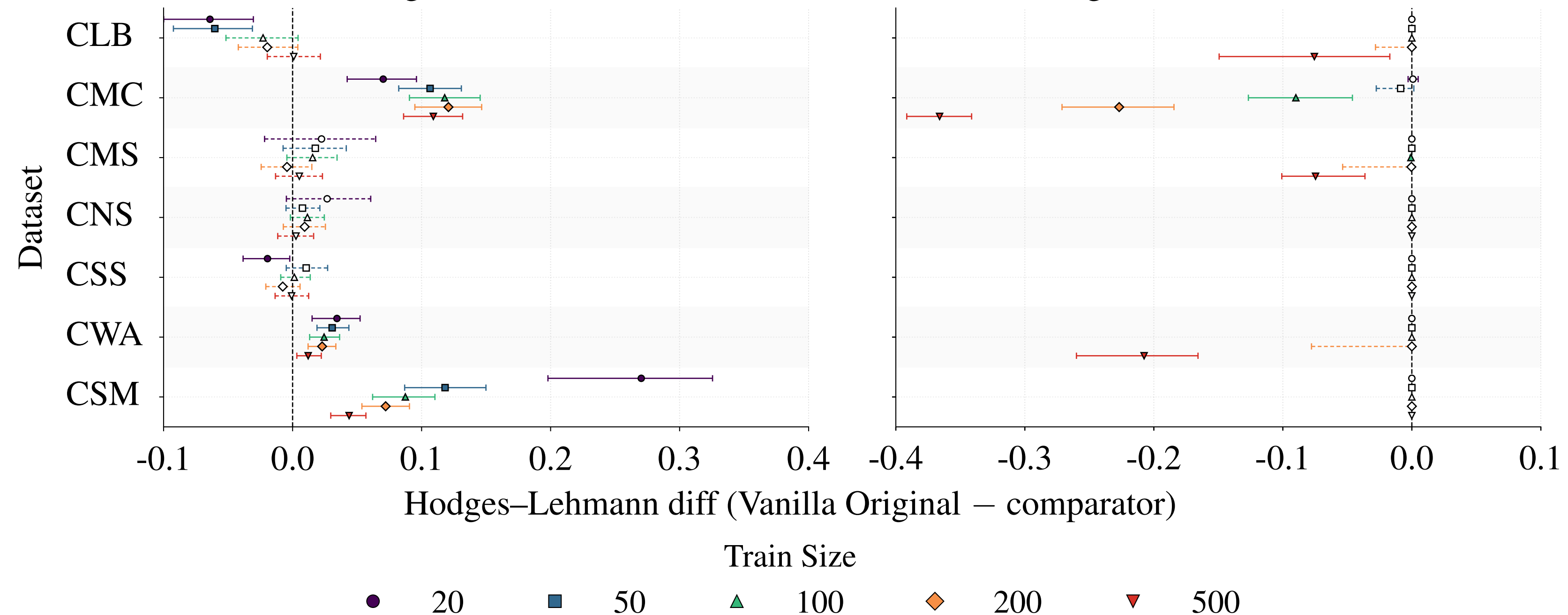
Vanilla Original vs oracle-PDAG
