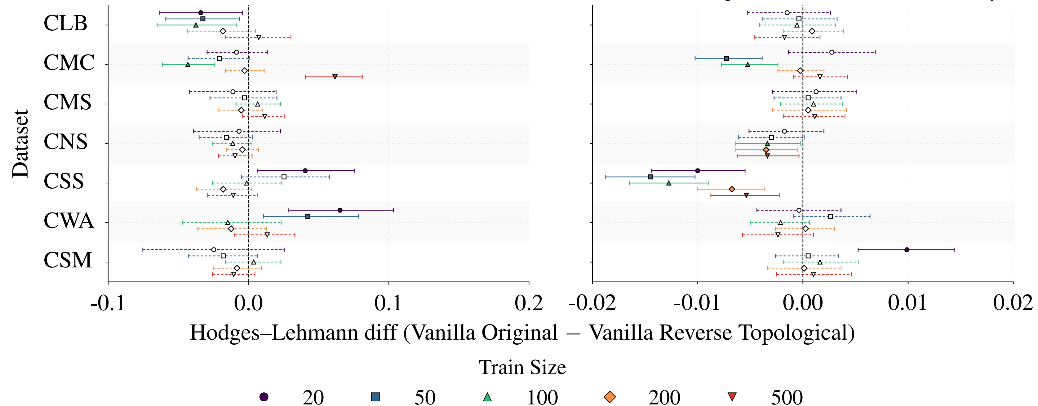
Nearest-Neighbor Adversarial Accuracy
