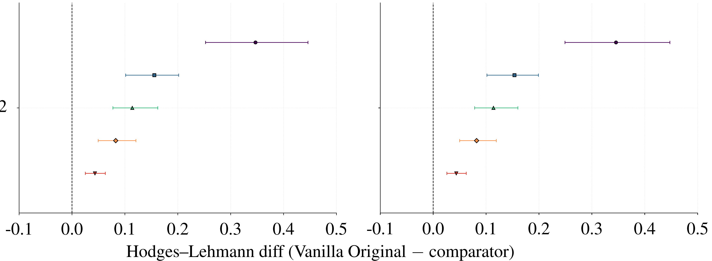
Vanilla Original vs DAG
