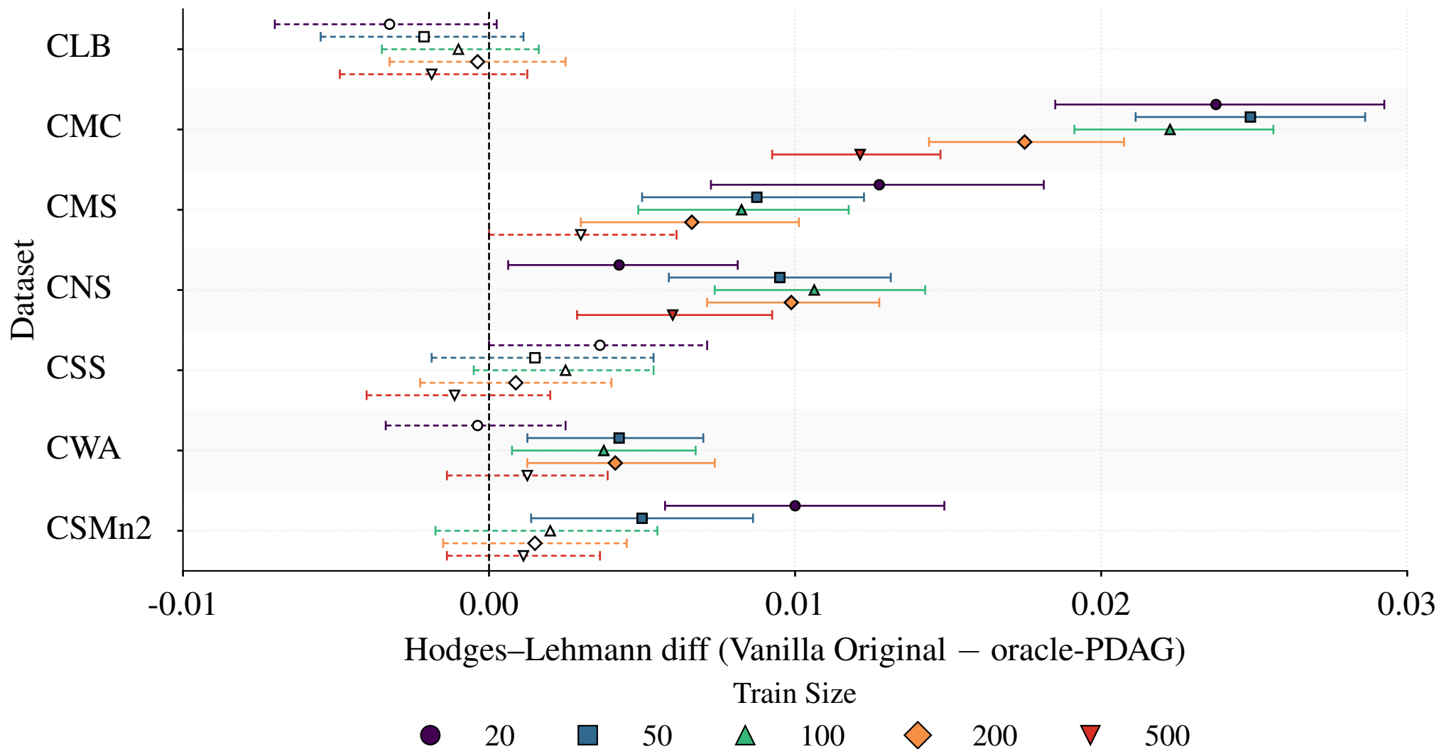
Vanilla Original vs oracle-PDAG |\text{Nearest-Neighbor Adversarial Accuracy} - 0.5|
